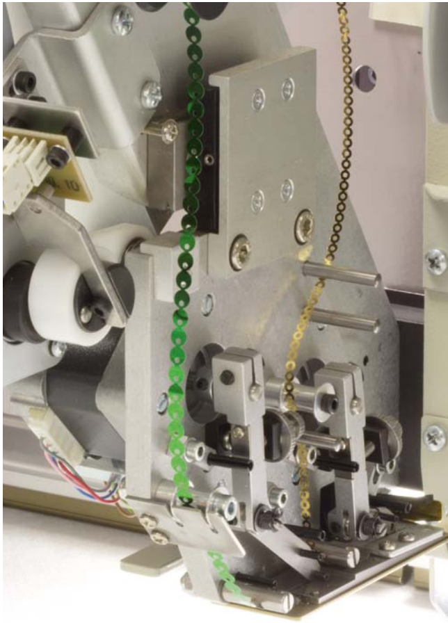
Sequin Device
