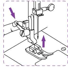
MATIC presser foot holder
