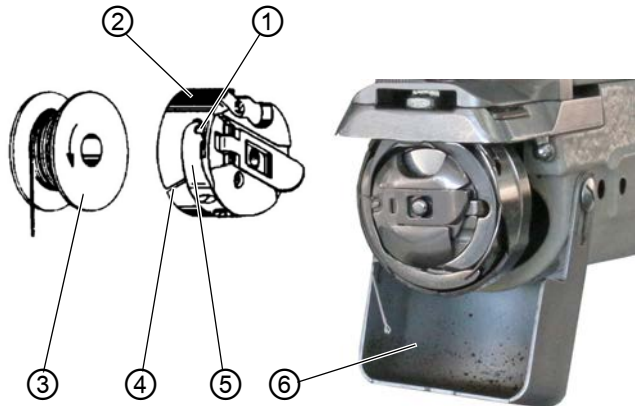
Image 12: Changer la canette
