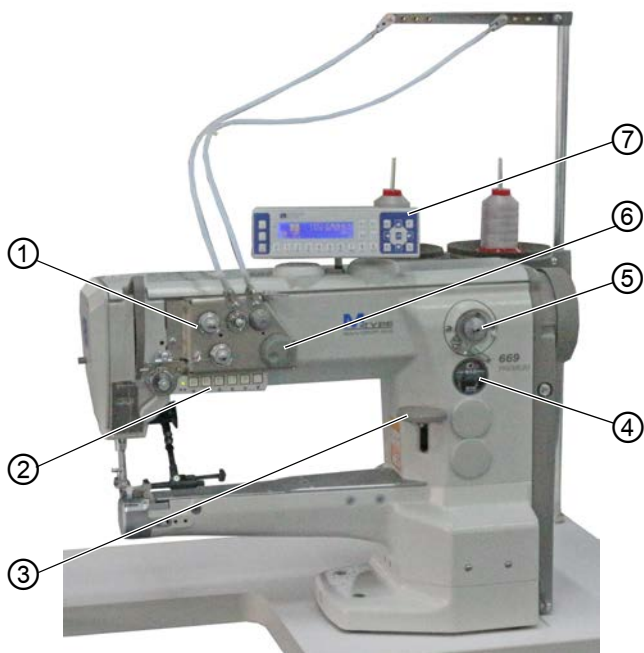
Image 1: Composants de la machine
