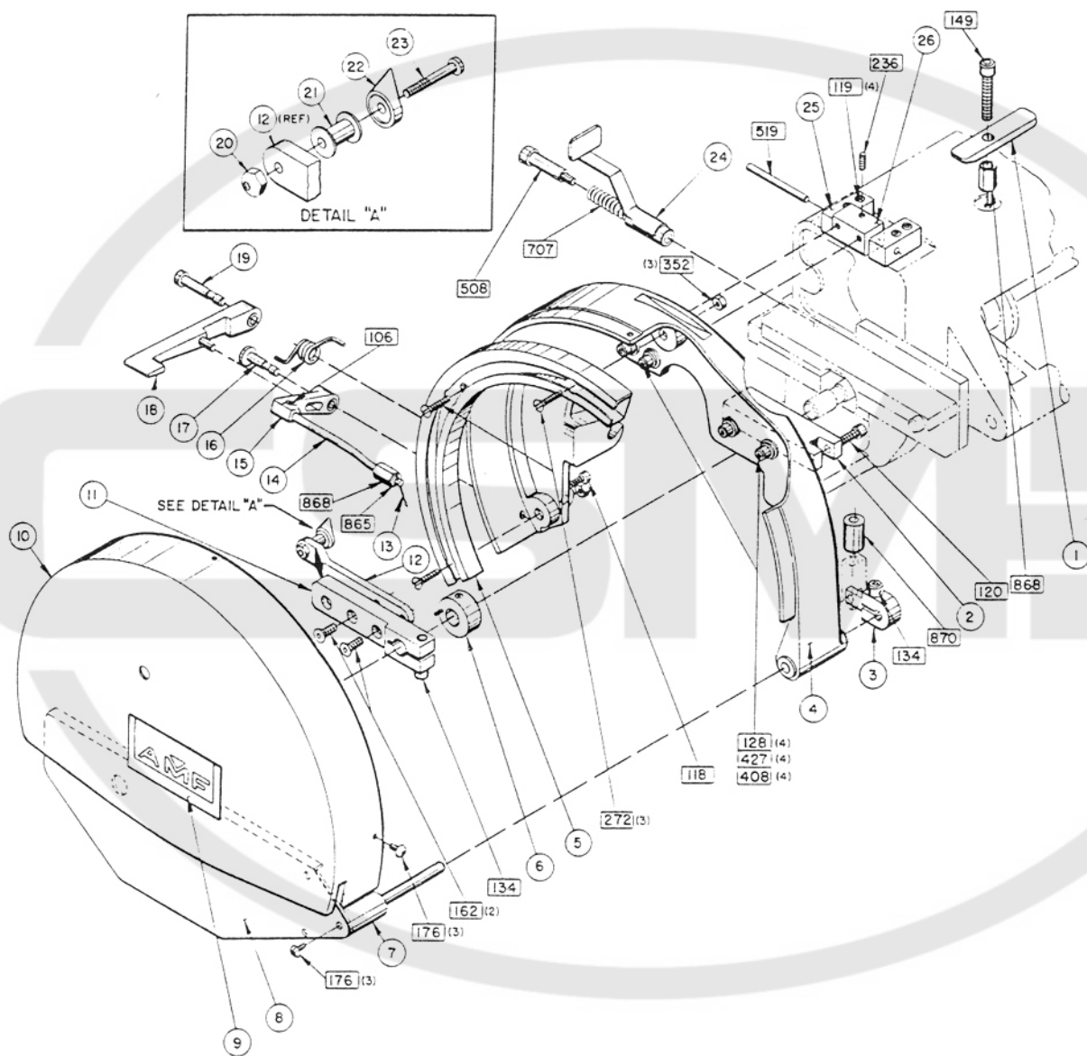
84-4 BUTTON STITCHING MACHINE UPPER LOOPER MECHANISM E.B.S.
