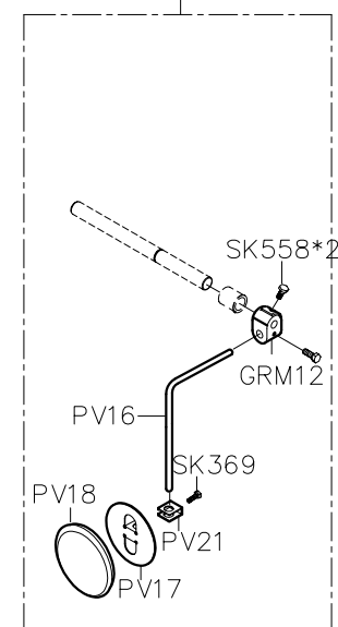
PARTS LIST FOR TY (1) GROUP
