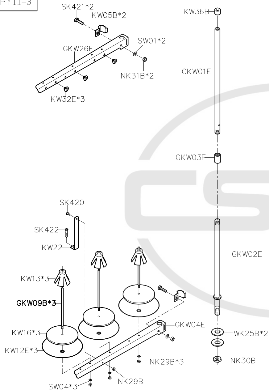
PARTS LIST FOR THREAD STAND GROUP
