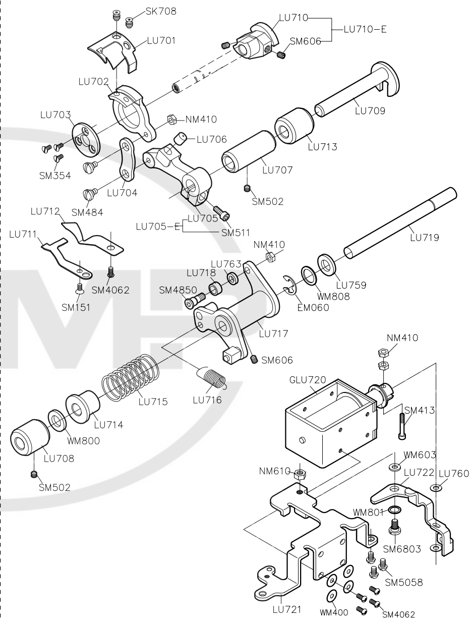
PARTS LIST FOR LU (1) GROUP
