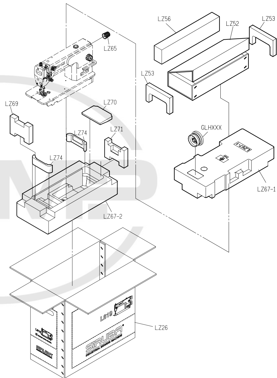
PARTS LIST FOR LZ GROUP
