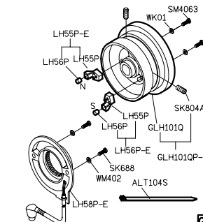
PARTS LIST FOR LH (2) GROUP
