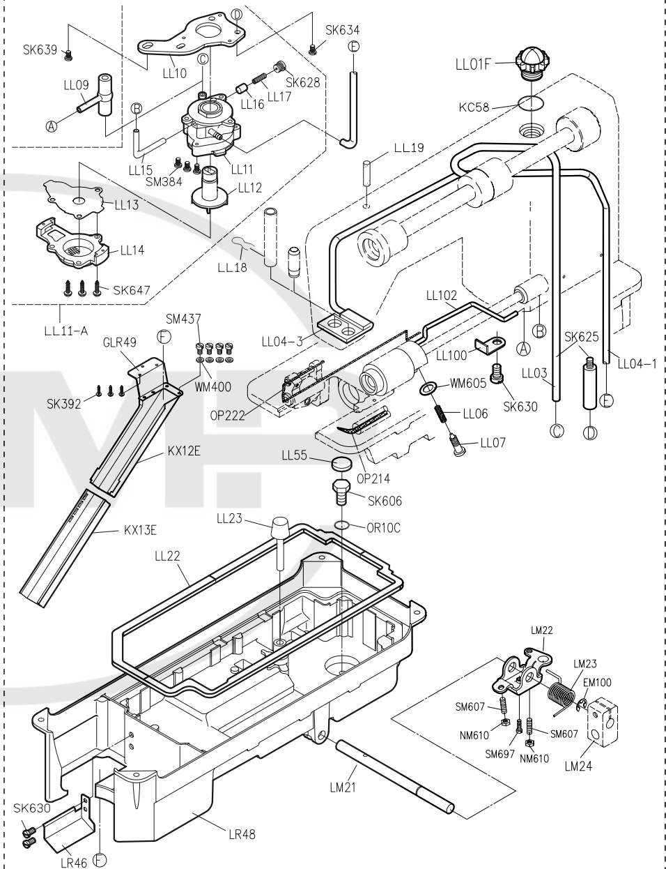
PARTS LIST FOR LL GROUP
