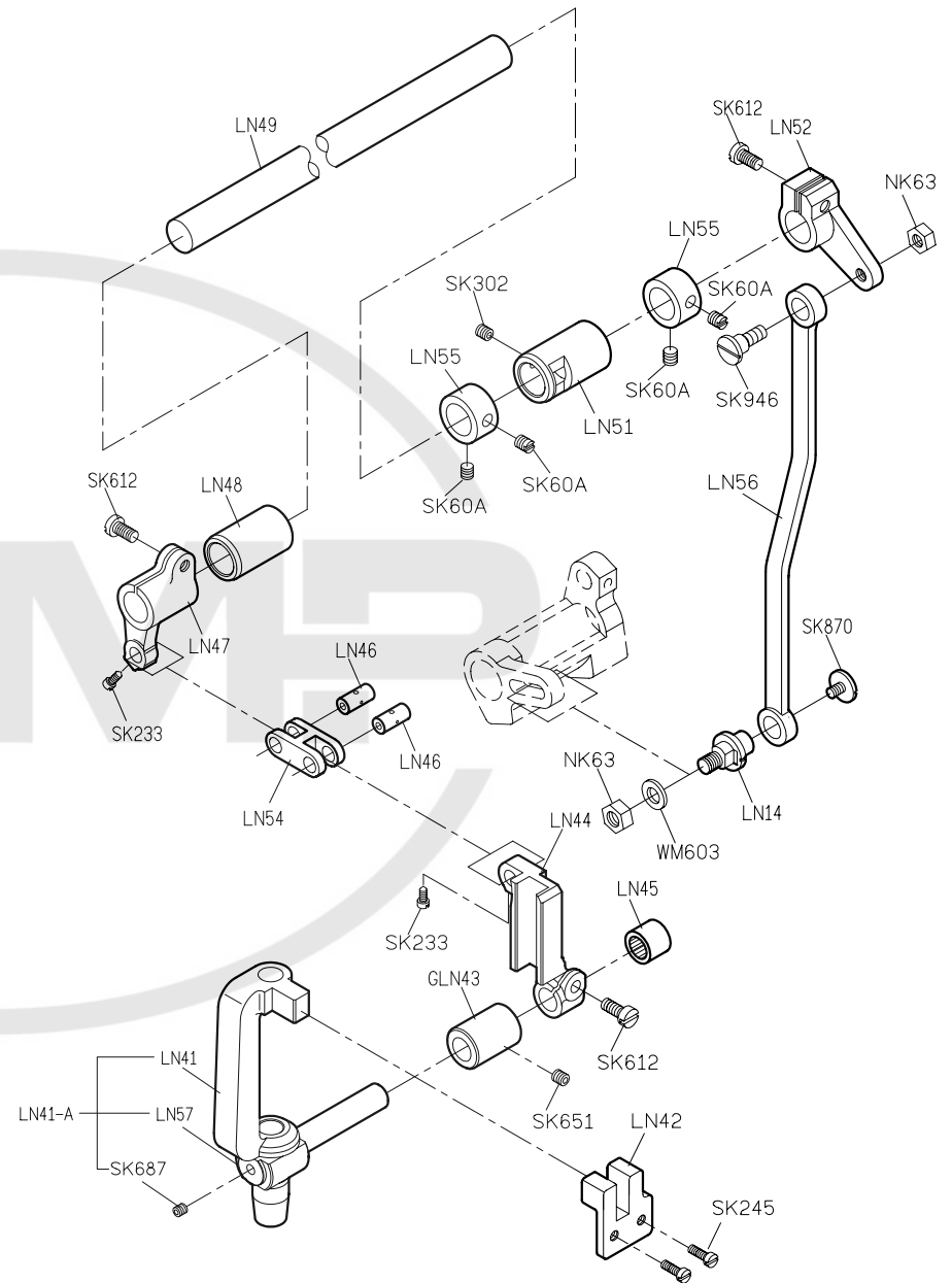
PARTS LIST FOR LN GROUP
