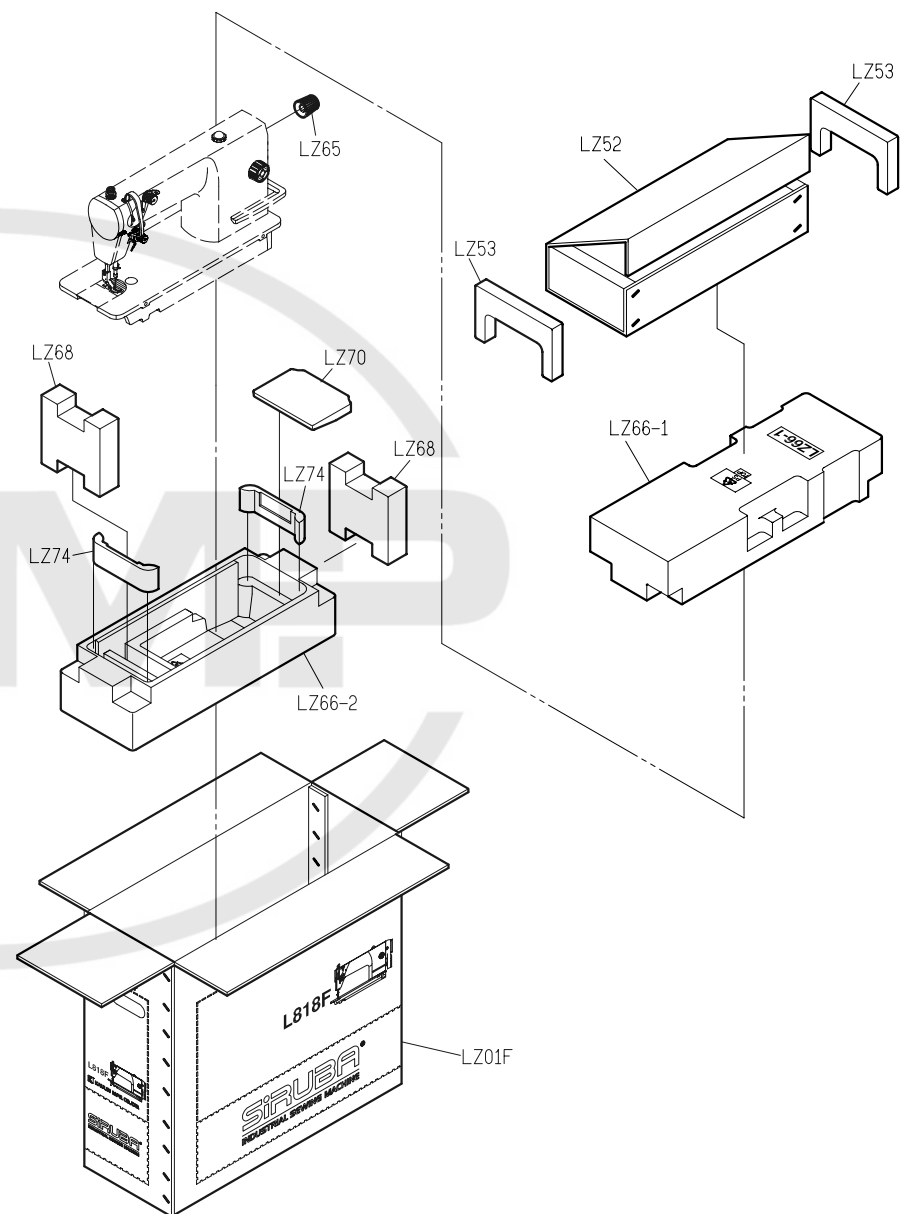
PARTS LIST FOR LZ GROUP
