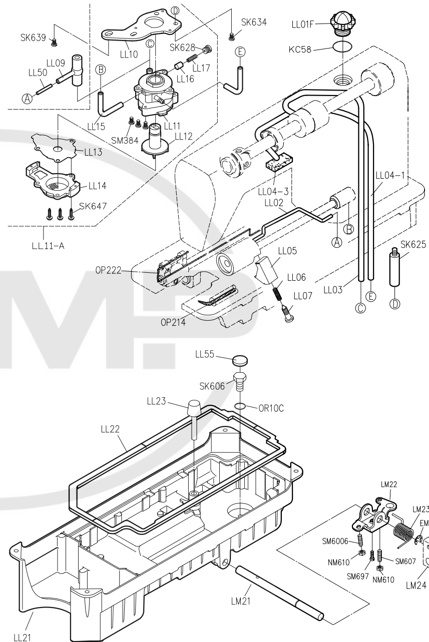
PARTS LIST FOR LL GROUP
