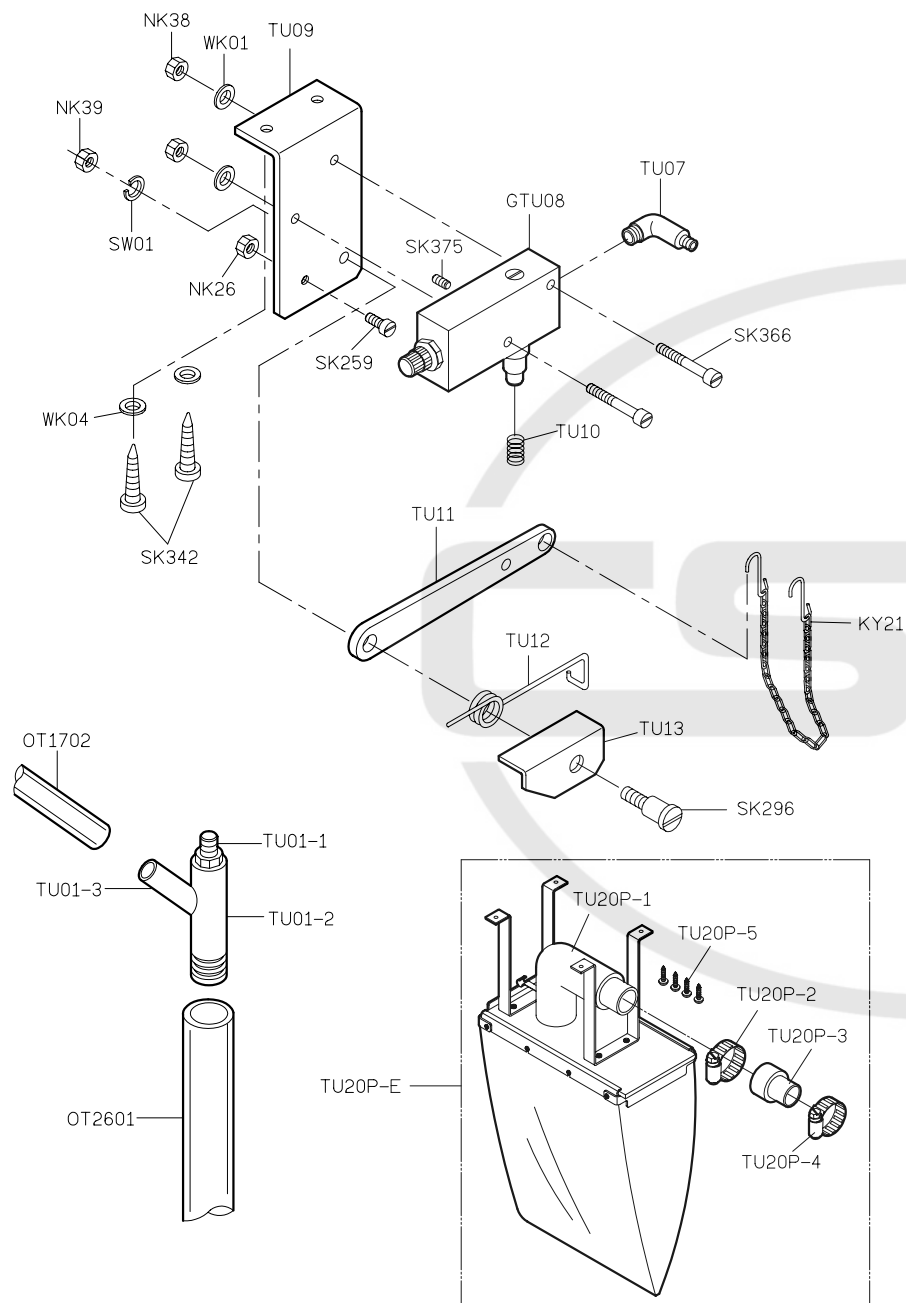
PARTS LIST FOR TU GROUP
