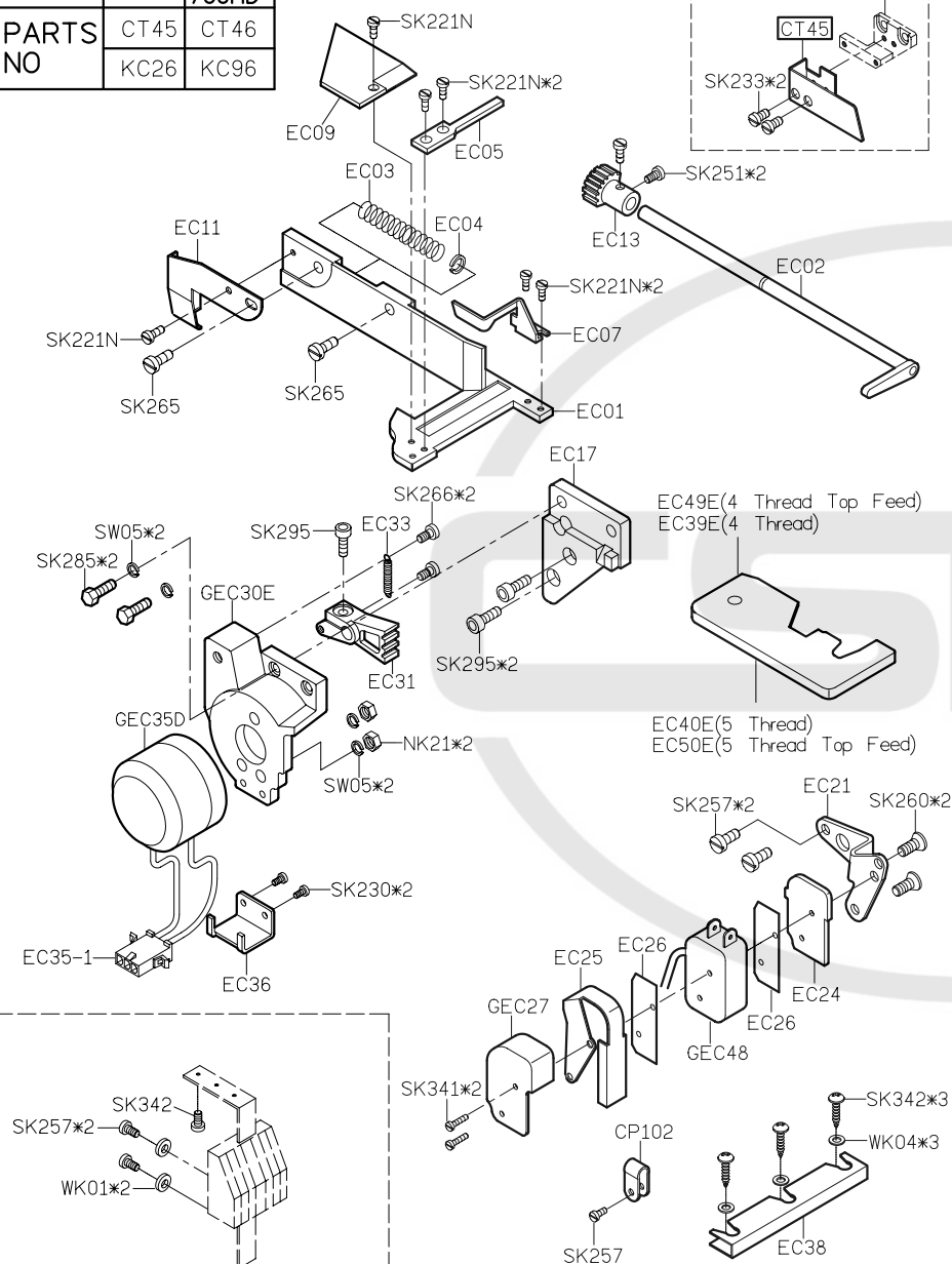
PARTS LIST FOR EC (1) GROUP
