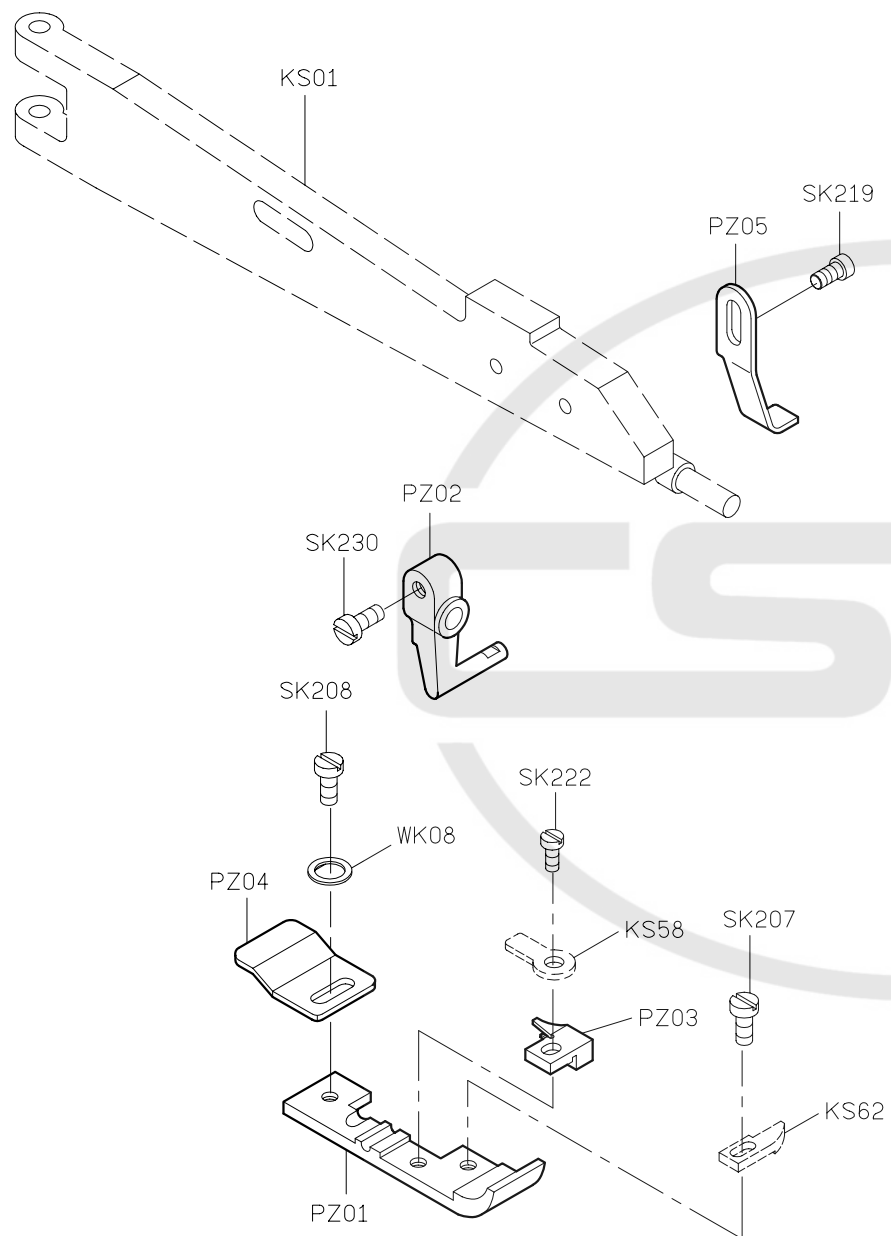
PARTS LIST FOR PZ GROUP
