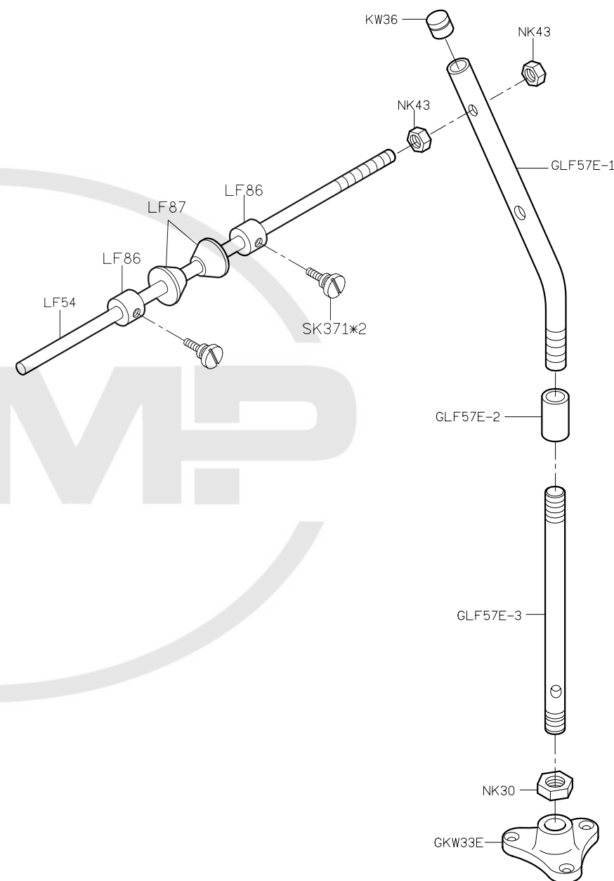
PARTS LIST FOR LS GROUP
