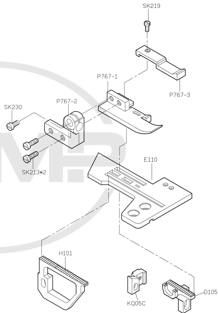
PARTS LIST FOR TW GROUP
