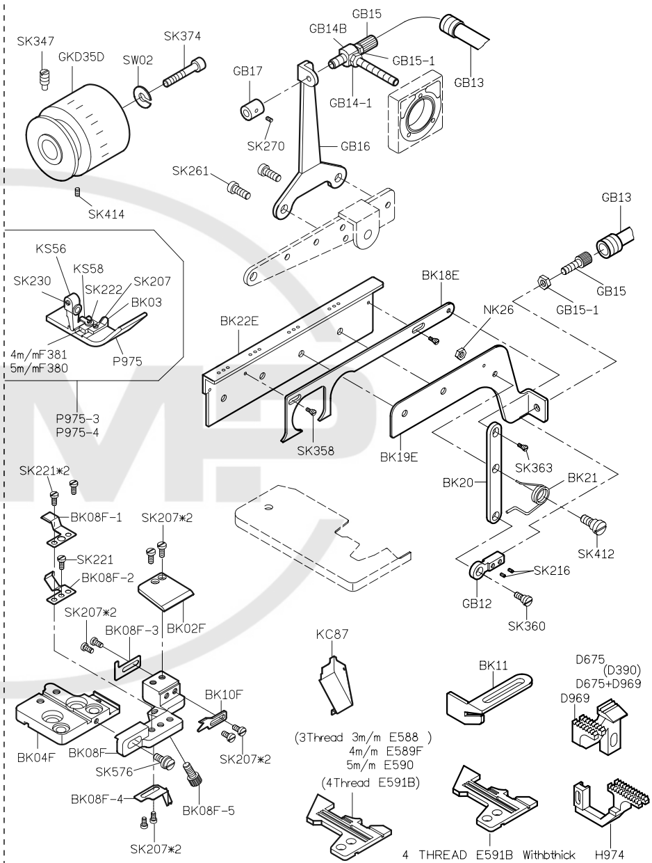
PARTS LIST FOR BK-F GROUP
