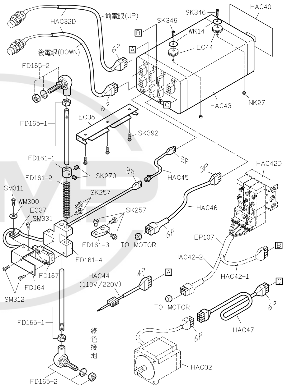
PARTS LIST FOR HAC (7) GROUP
