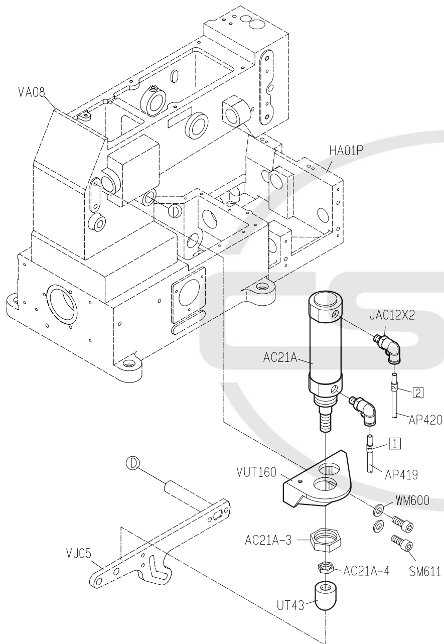
PARTS LIST FOR HAC (6) GROUP
