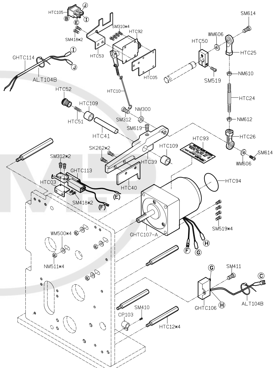
PARTS LIST FOR HTC (2) GROUP
