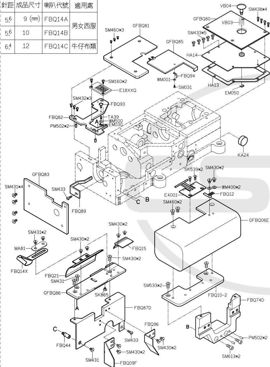
PARTS LIST FOR FBQ (1) GROUP
