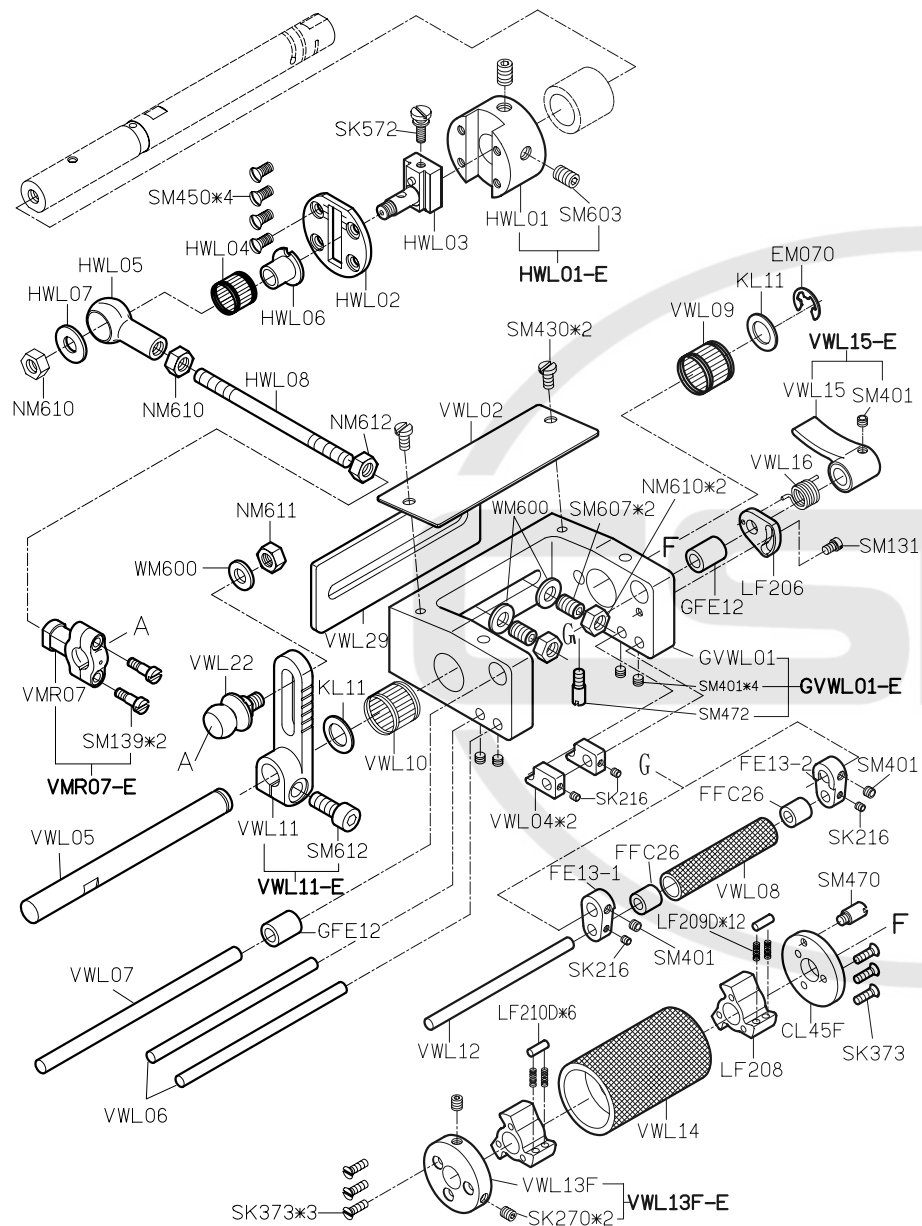
PARTS LIST FOR HWL (1) GROUP
