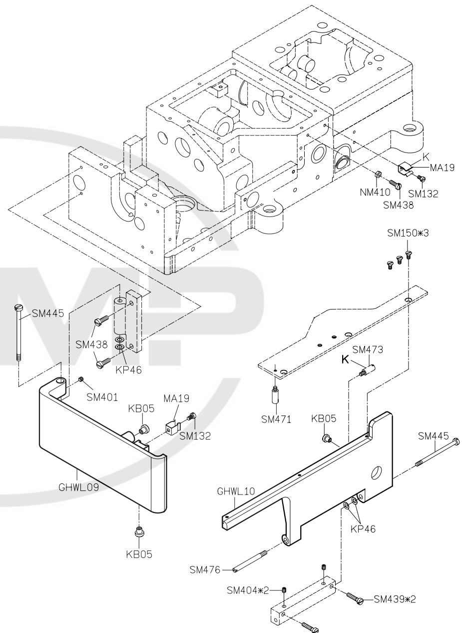
PARTS LIST FOR HWL (2) GROUP
