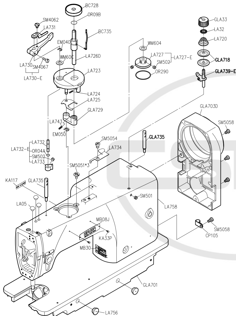
PARTS LIST FOR LA (1) GROUP
