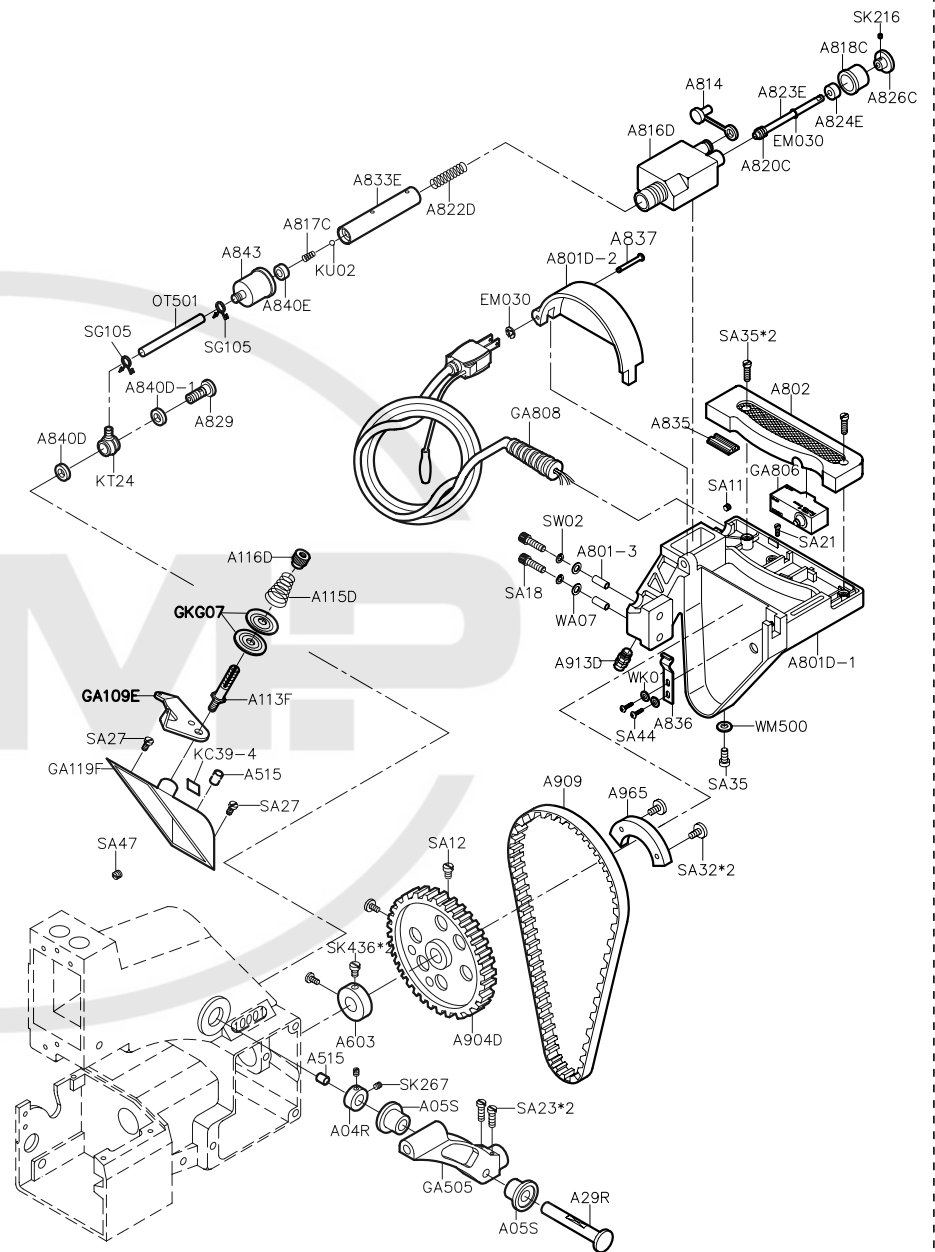
PARTS LIST FOR AA (2) GROUP
