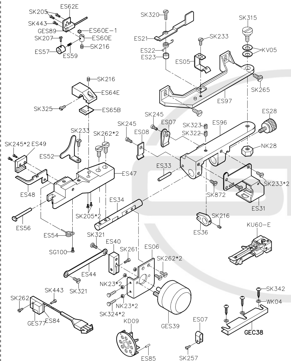
700FS ATTACHMENT
