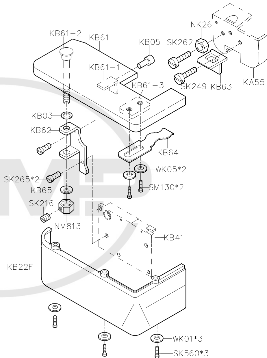
700FS ATTACHMENT
