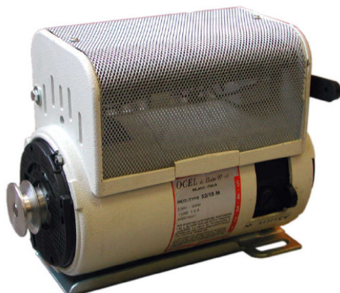
Motor Ocel/Moretti 70/18 220V - 250W 1/6-1/3PK (HP) 3500/600 RPM/Tm
