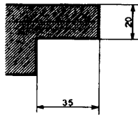
Section I-I
