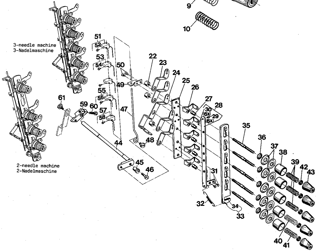
2-needle machine 2-Nadelmaschine
