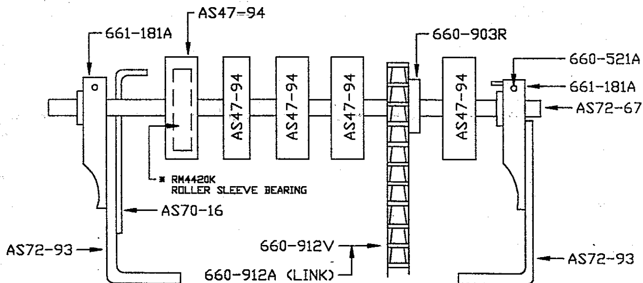
TAILSHAFT-RIGHT LOADING
