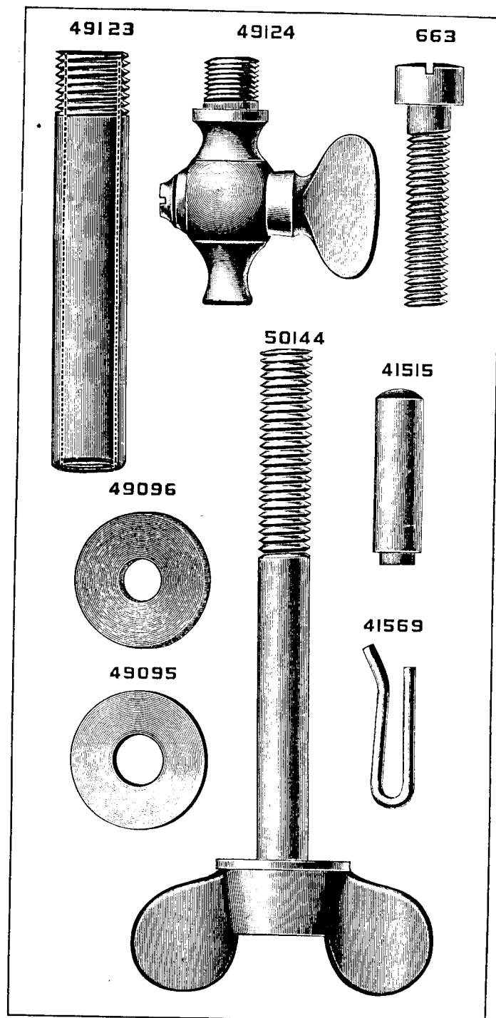
PLATE 6199—FULL SIZE
