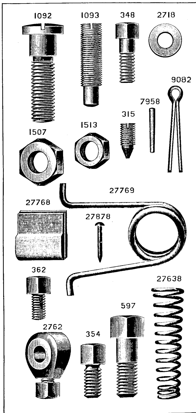
PLATE 2642—FULL SIZE
