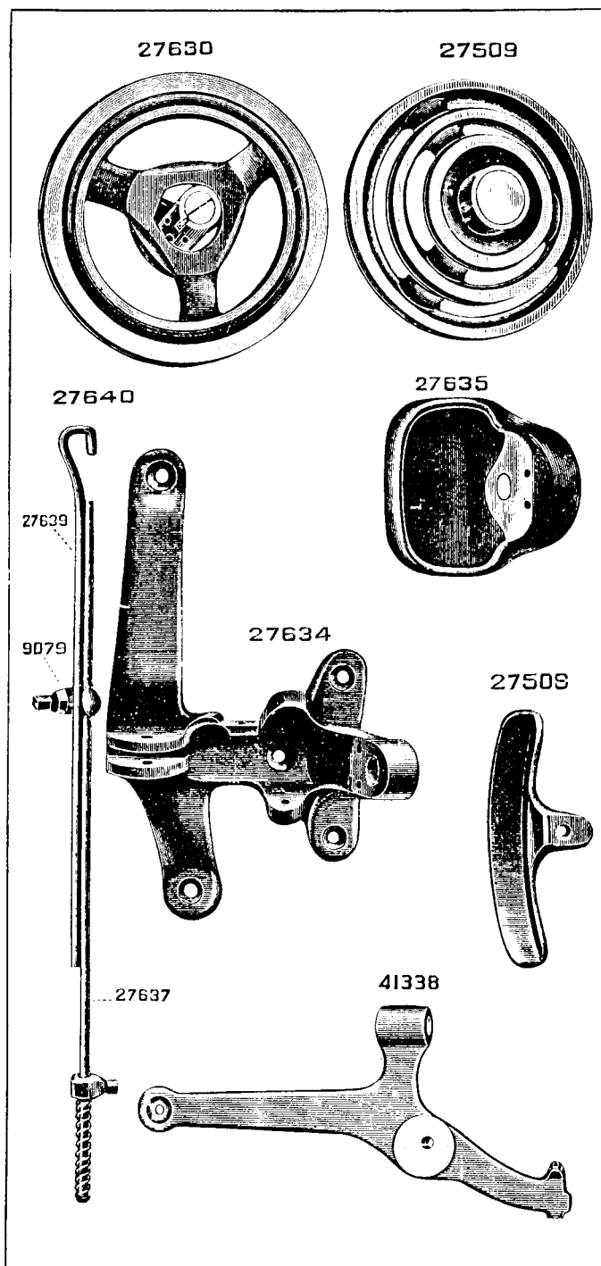
PLATE 362—ONE-FOURTH SIZE
