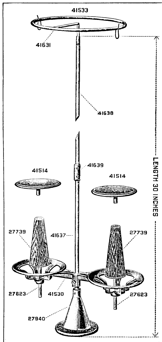
PLATE 2837—ONE-FOURTH SIZE
