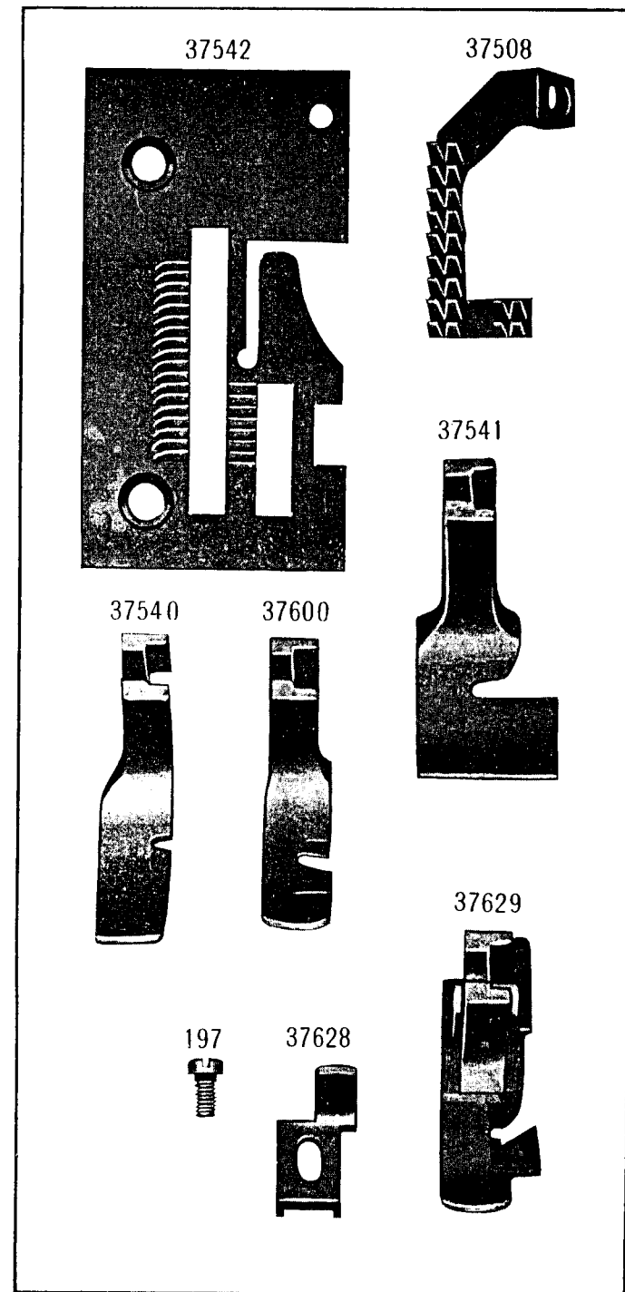
PLATE 6714—FULL SIZE
