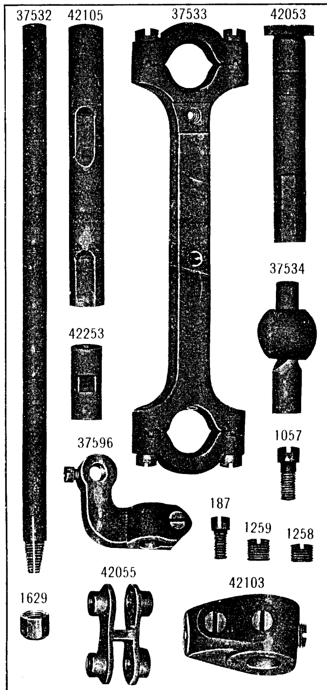
PLATE 6721—FULL SIZE
