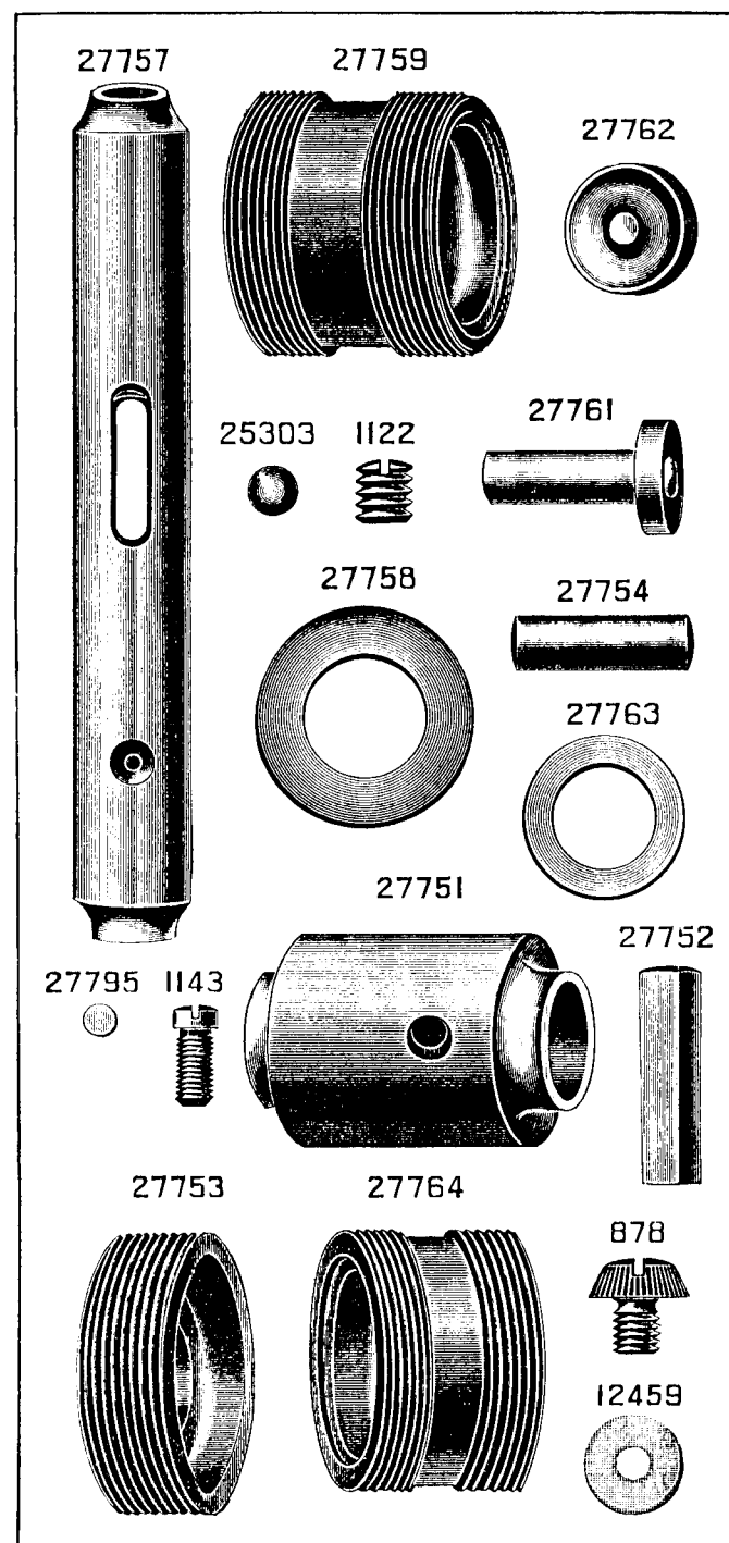
PLATE 2641—FULL SIZE
