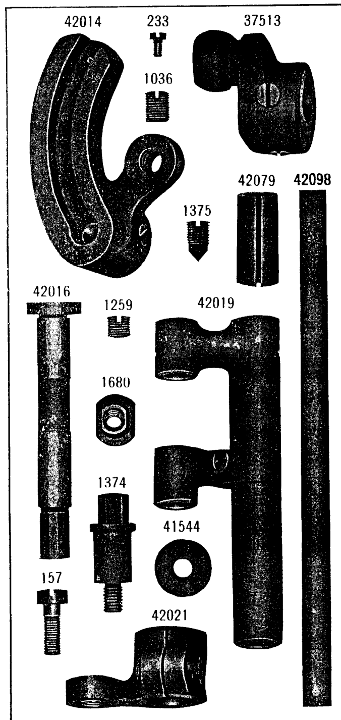
PLATE 6718--FULL SIZE
