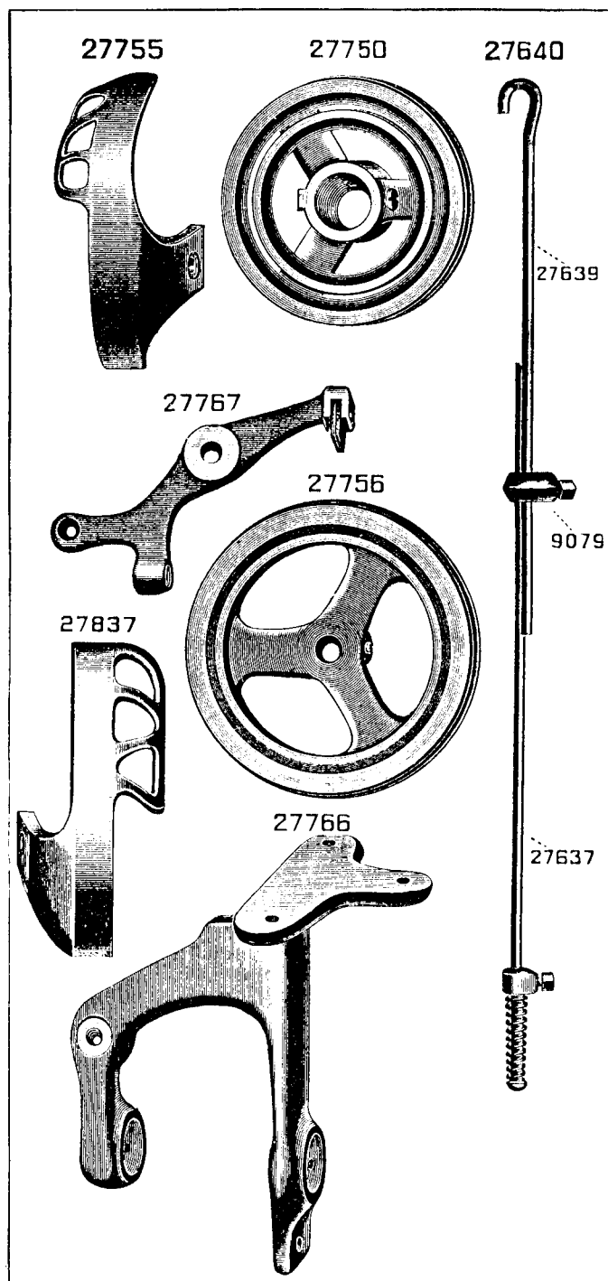
PLATE 2640—ONE-FOURTH SIZE
