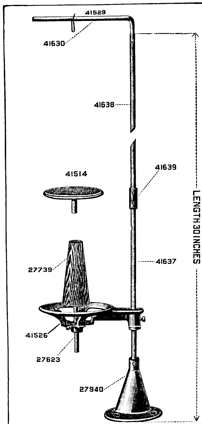
PLATE 2836—ONE-FOURTH SIZE
