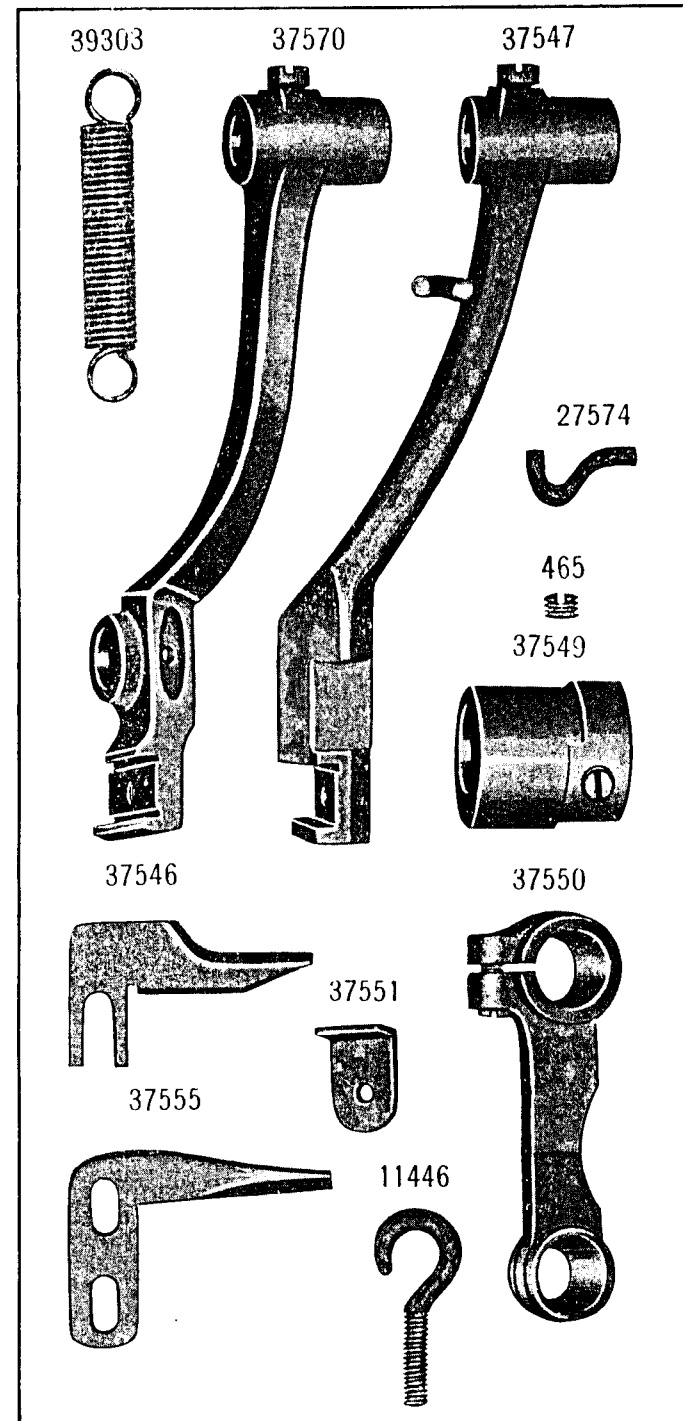
PLATE 6724—FULL SIZE
