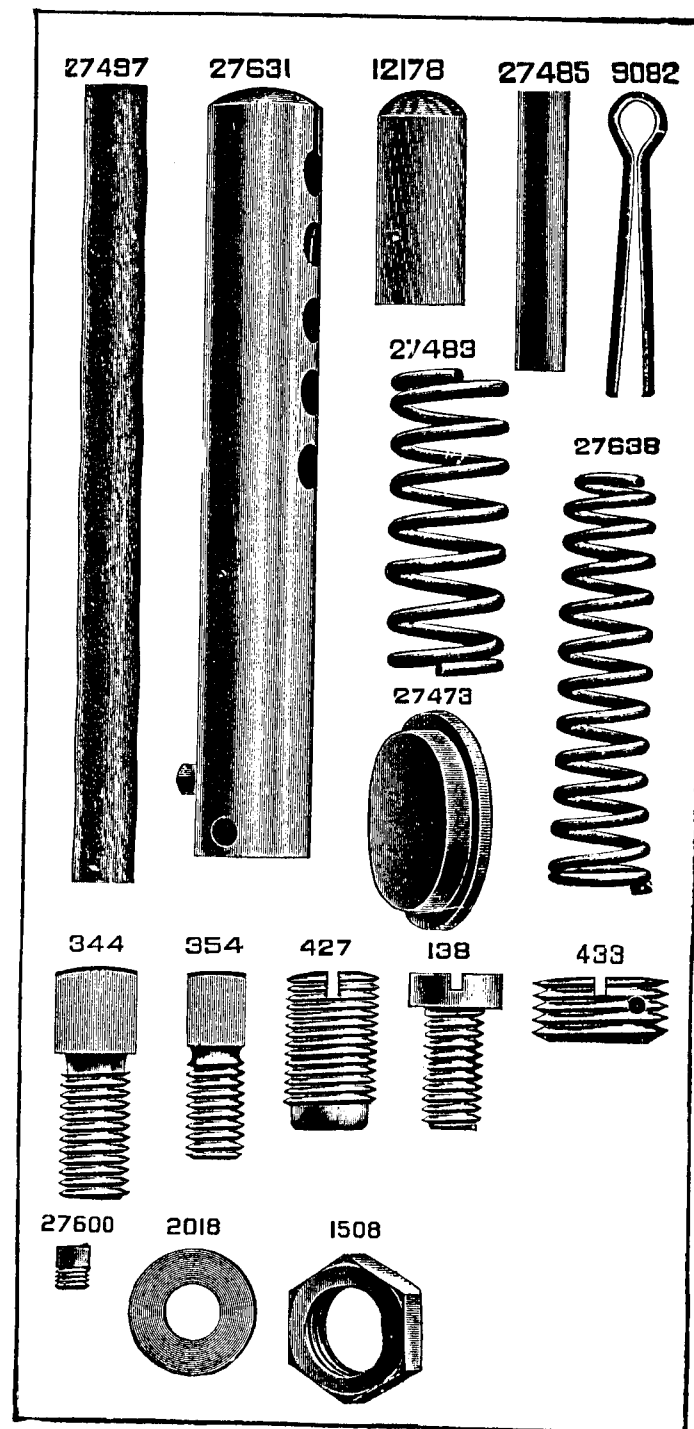
PLATE 1101—FULL SIZE
