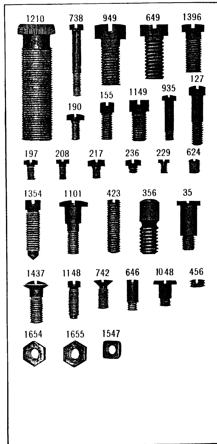
PLATE 6730—FULL SIZE
