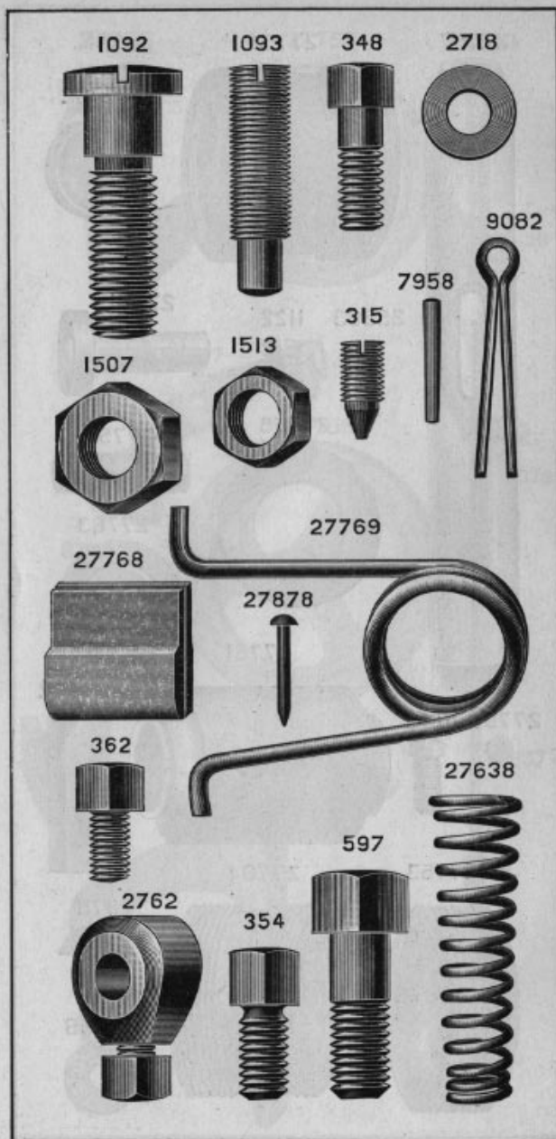
PLATE 2642—FULL SIZE
