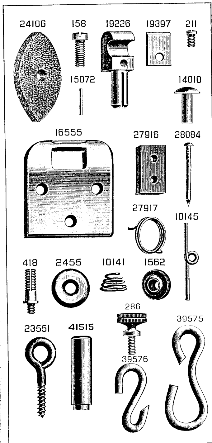
PLATE 4024—FULL SIZE
