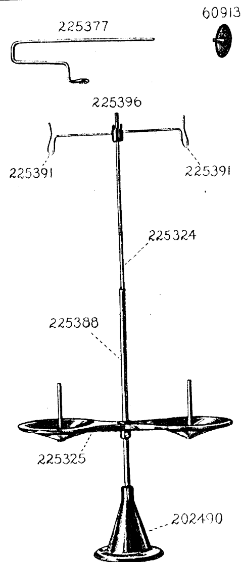
PLATE 14263—ONE-SIXTH SIZE
