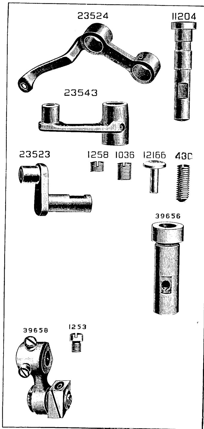
PLATE 4023—FULL SIZE
