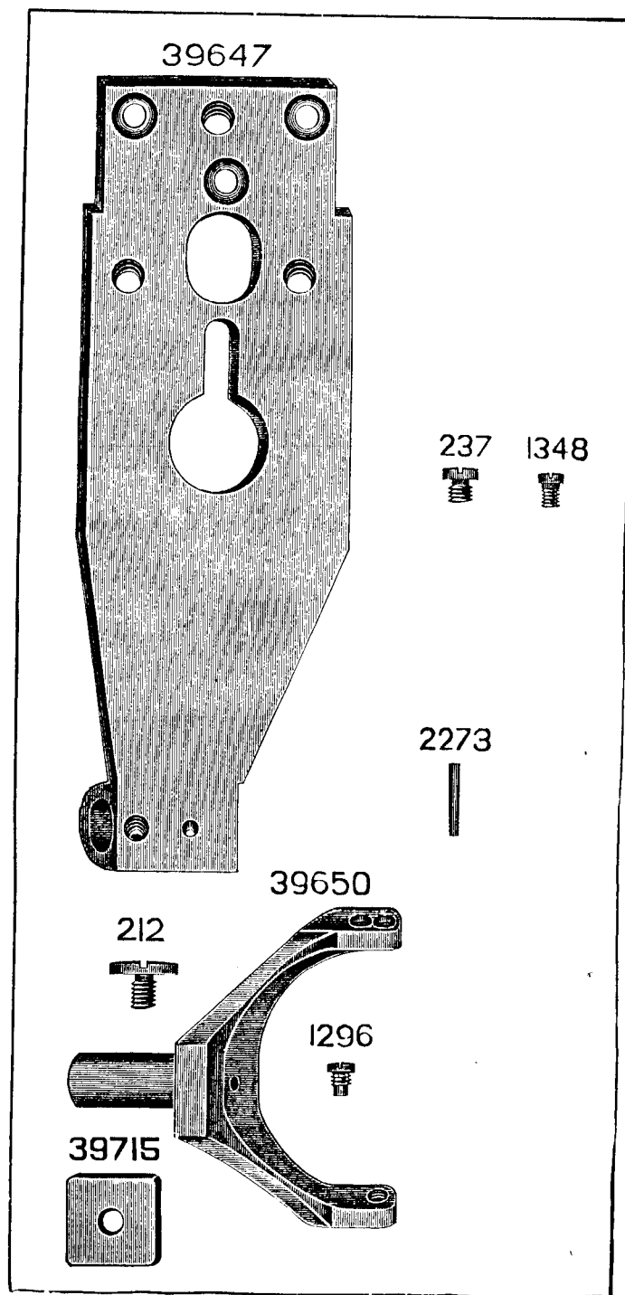
PLATE 4066—FULL SIZE
