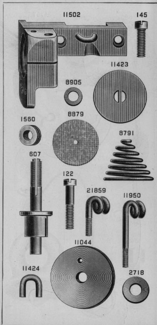
PLATE 4517—FULL SIZE
