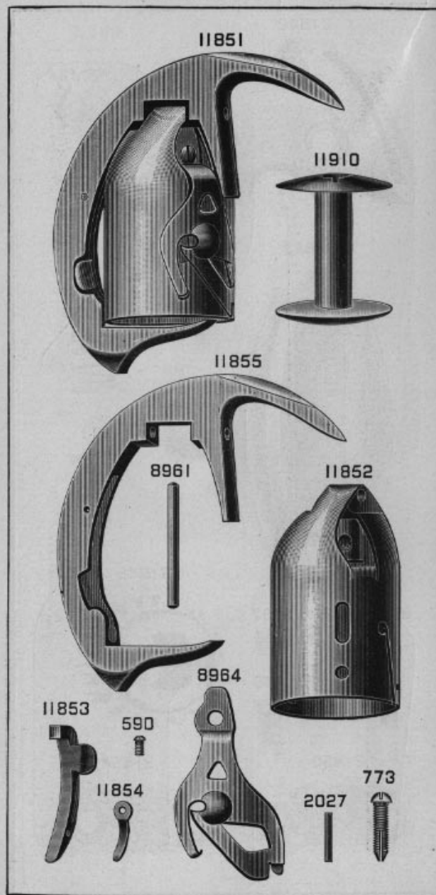
PLATE 4513—FULL SIZE
