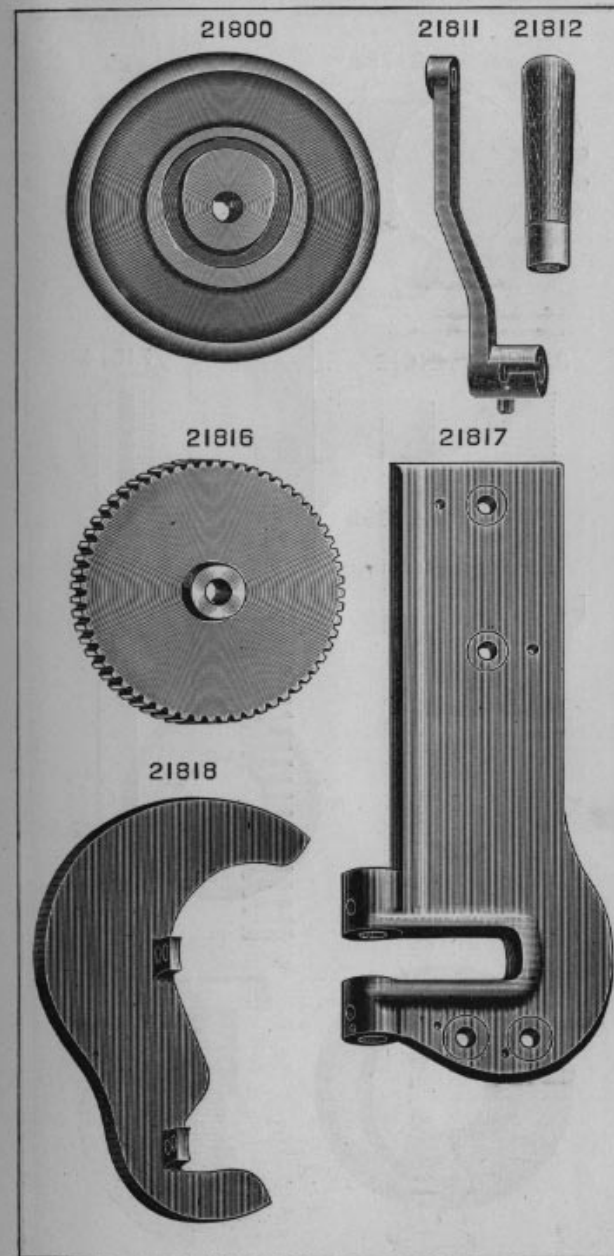
PLATE 4504—ONE-FOURTH SIZE
