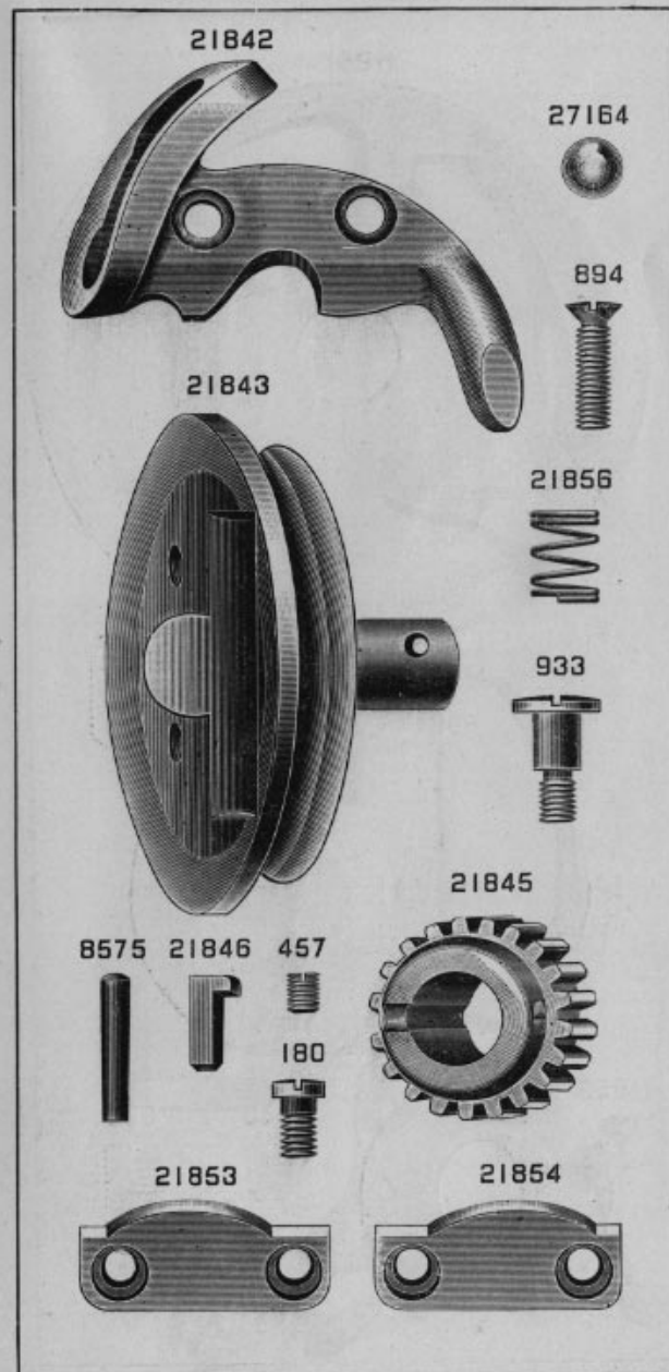
PLATE 4514—FULL SIZE
