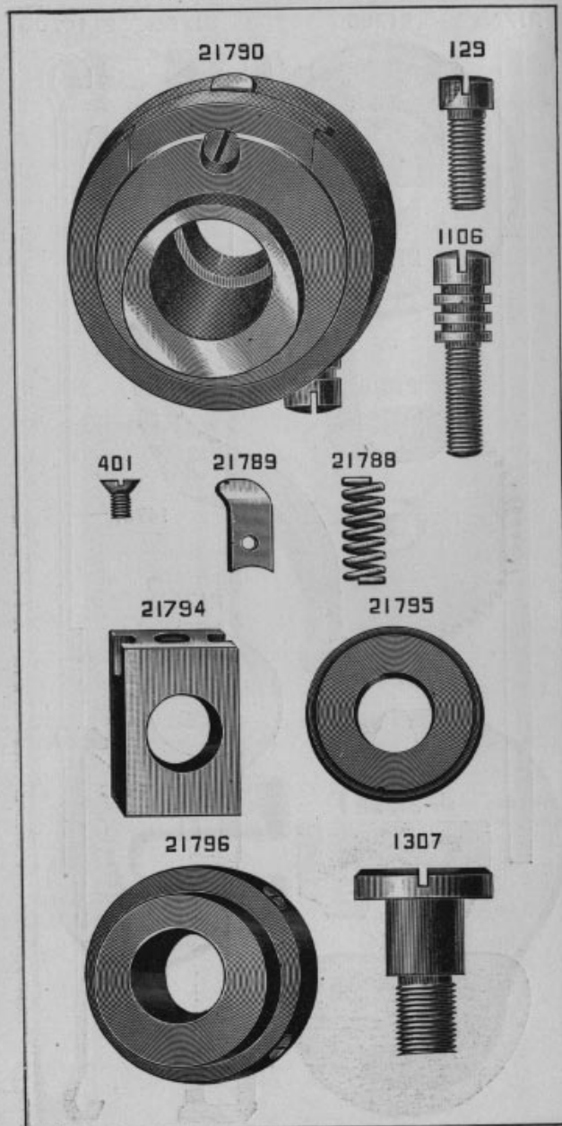
PLATE 4503—FULL SIZE
