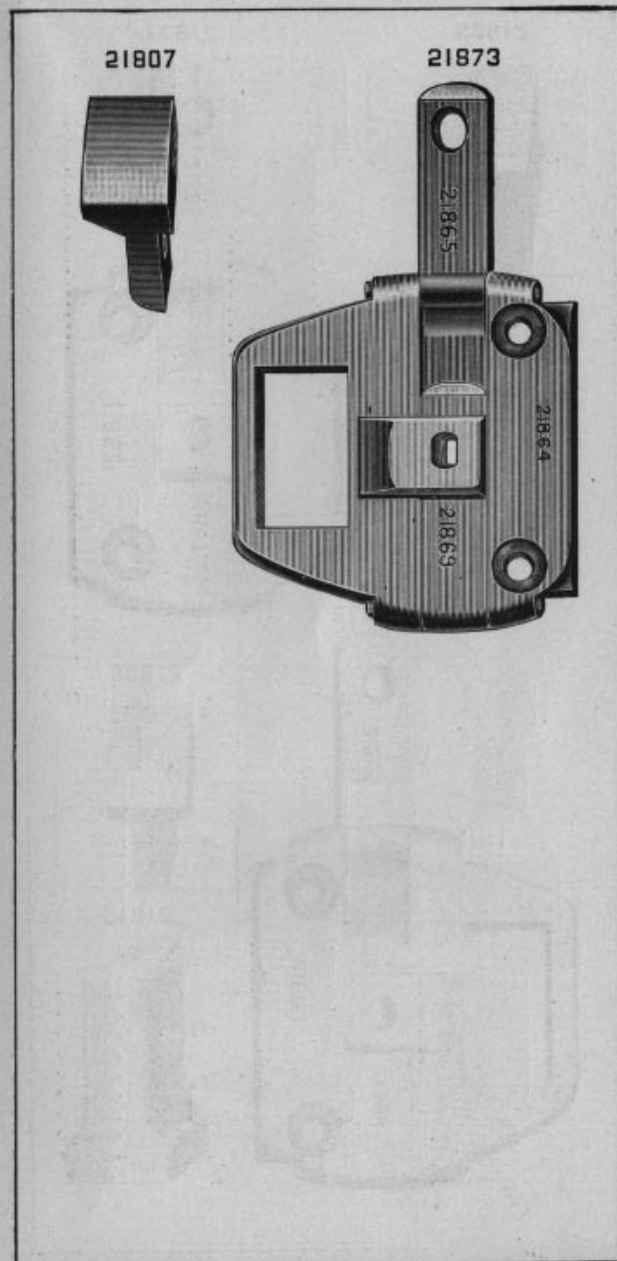
PLATE 4522—FULL SIZE
