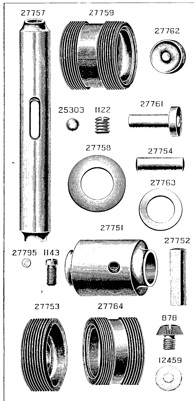
PLATE 2641—FULL SIZE
