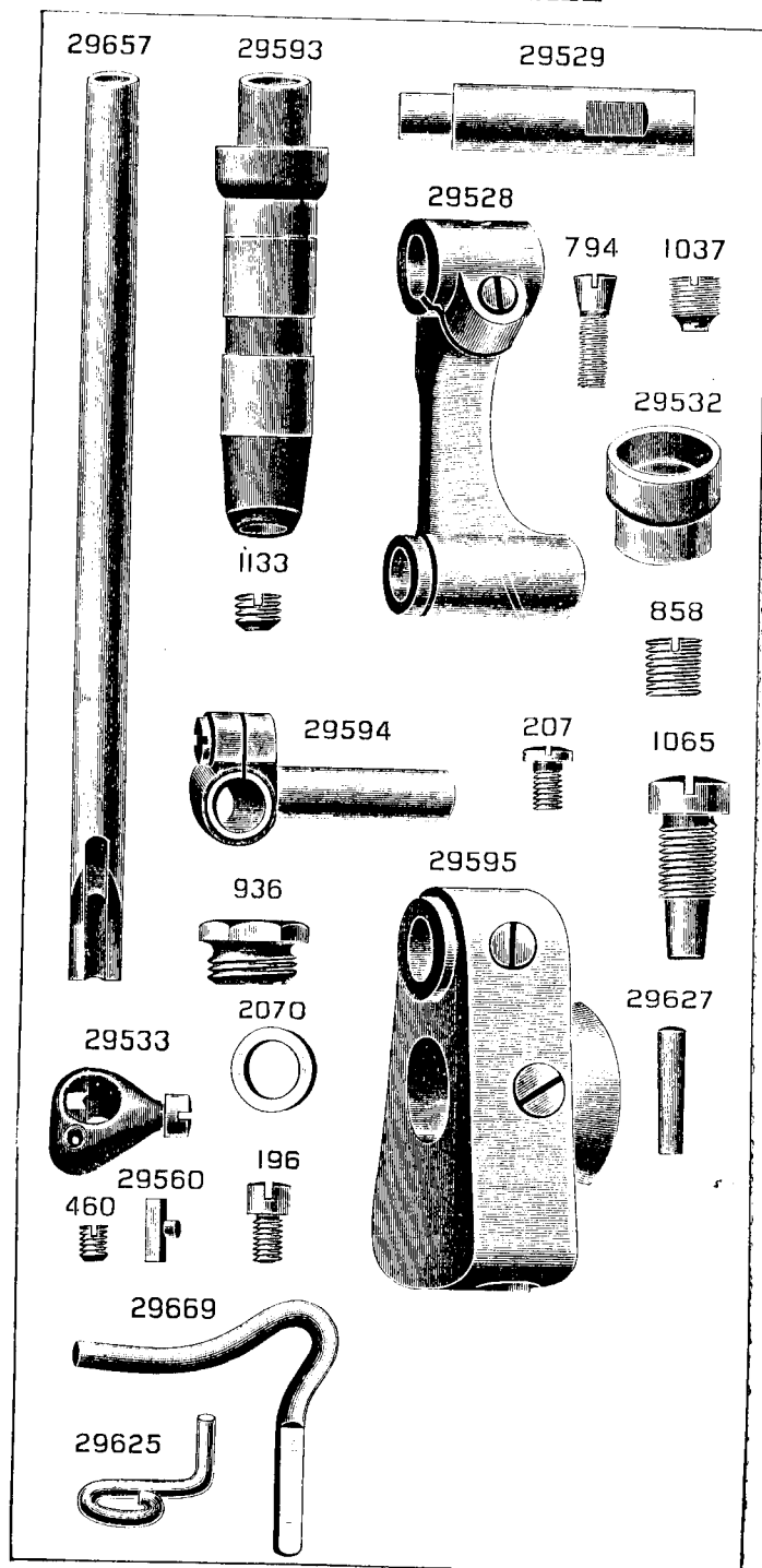
PLATE 3504—FULL SIZE
