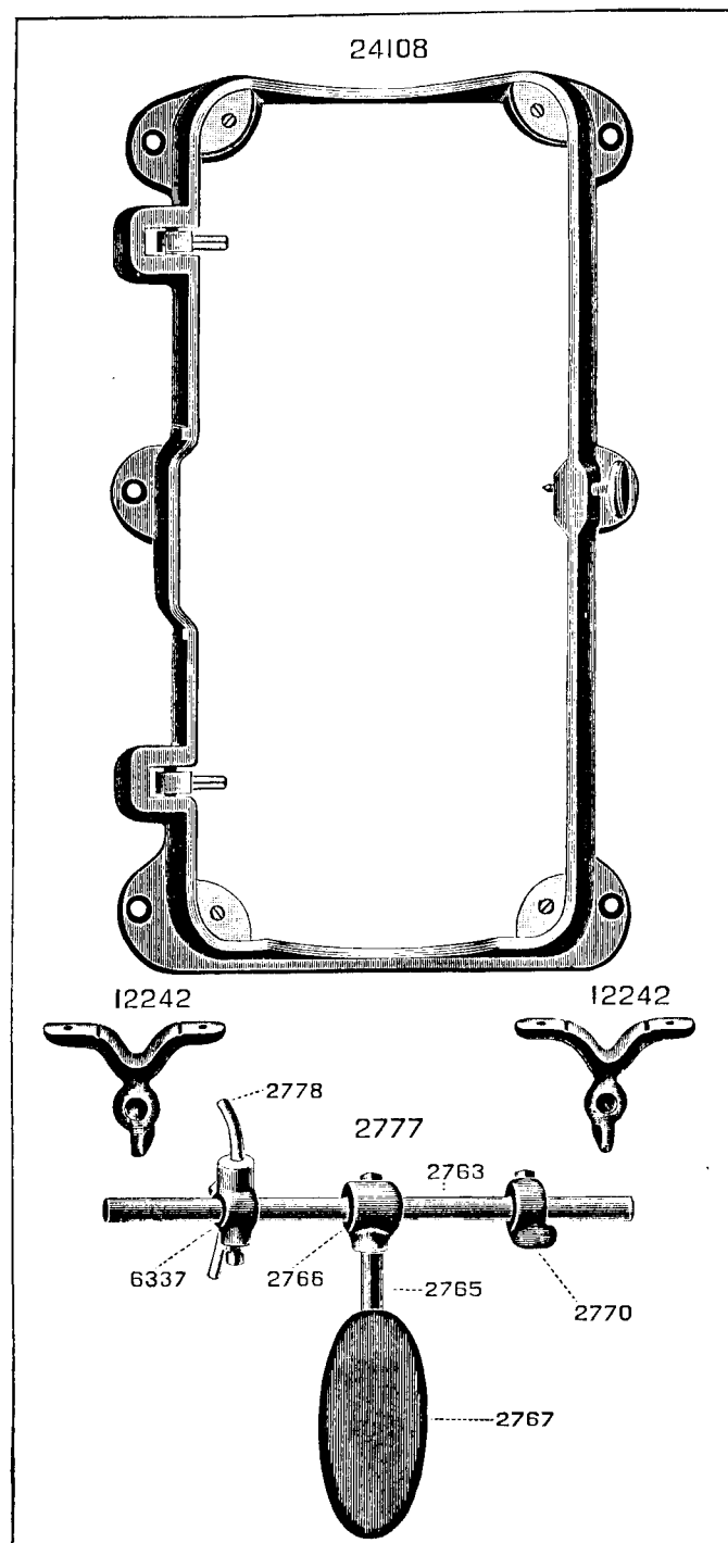
PLATE 3538—ONE-FOURTH SIZE
