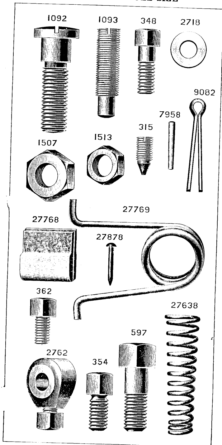
PLATE 2642—FULL SIZE
