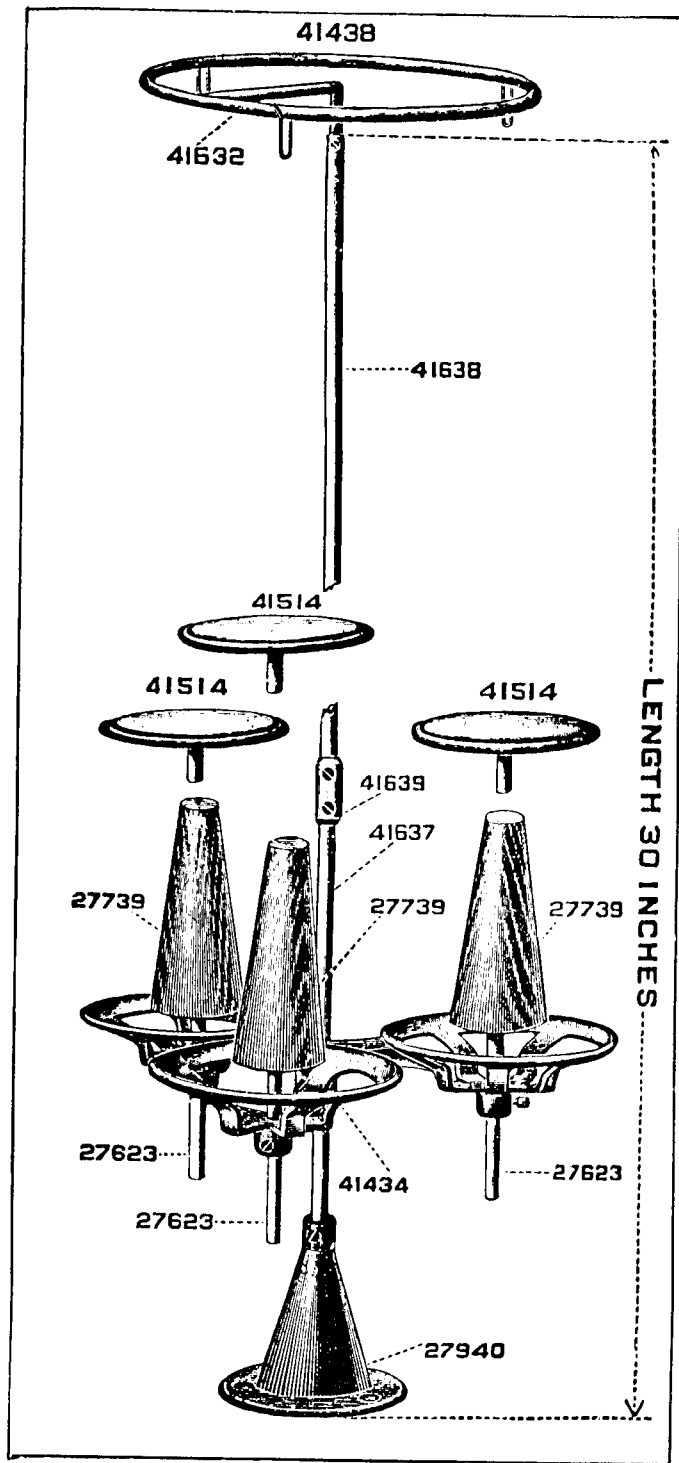
PLATE 5571—ONE-FOURTH SIZE
