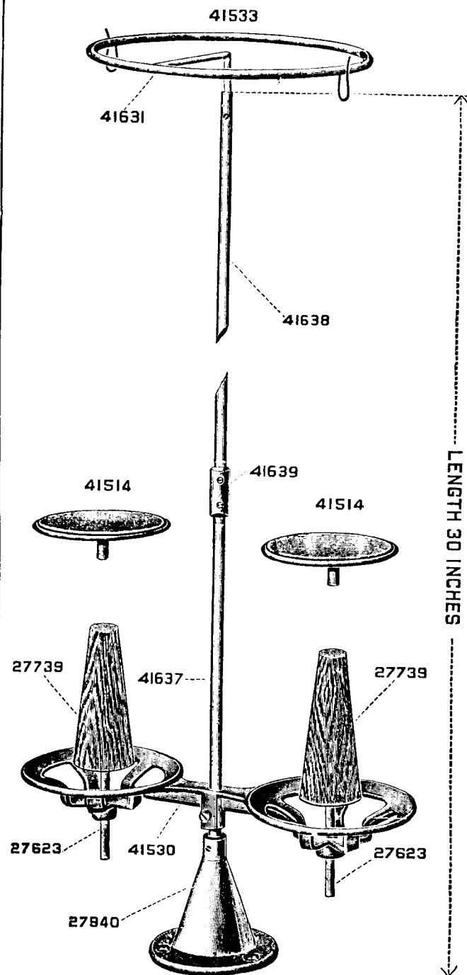
PLATE 2837—ONE-FOURTH SIZE
