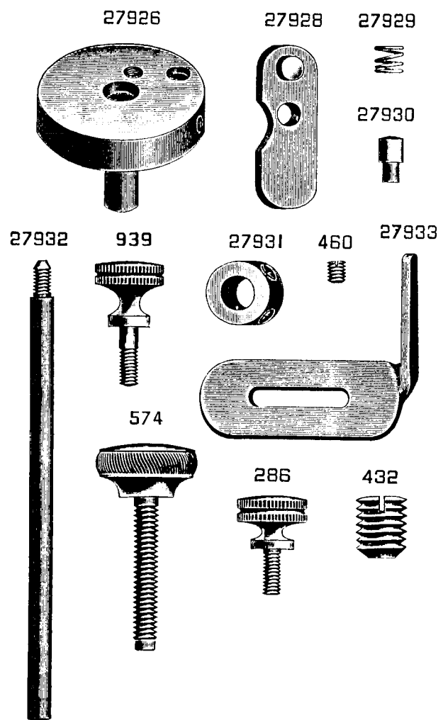
PLATE 4875—FULL SIZE
