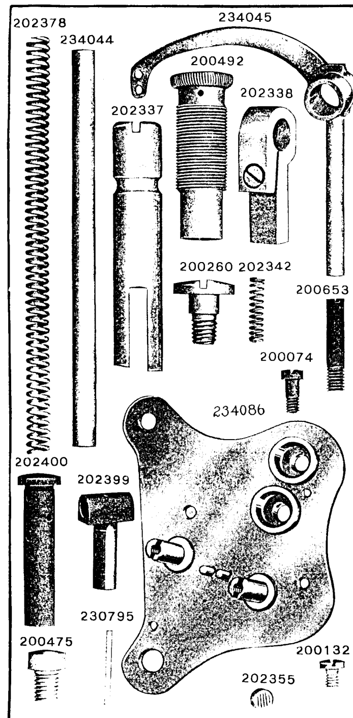
PLATE 13307-FULL SIZE
