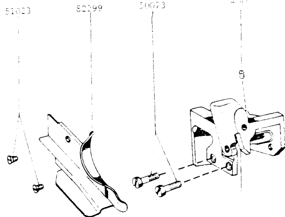
Knife (movable) Lever Cover and Pressor Bar Housing complete
