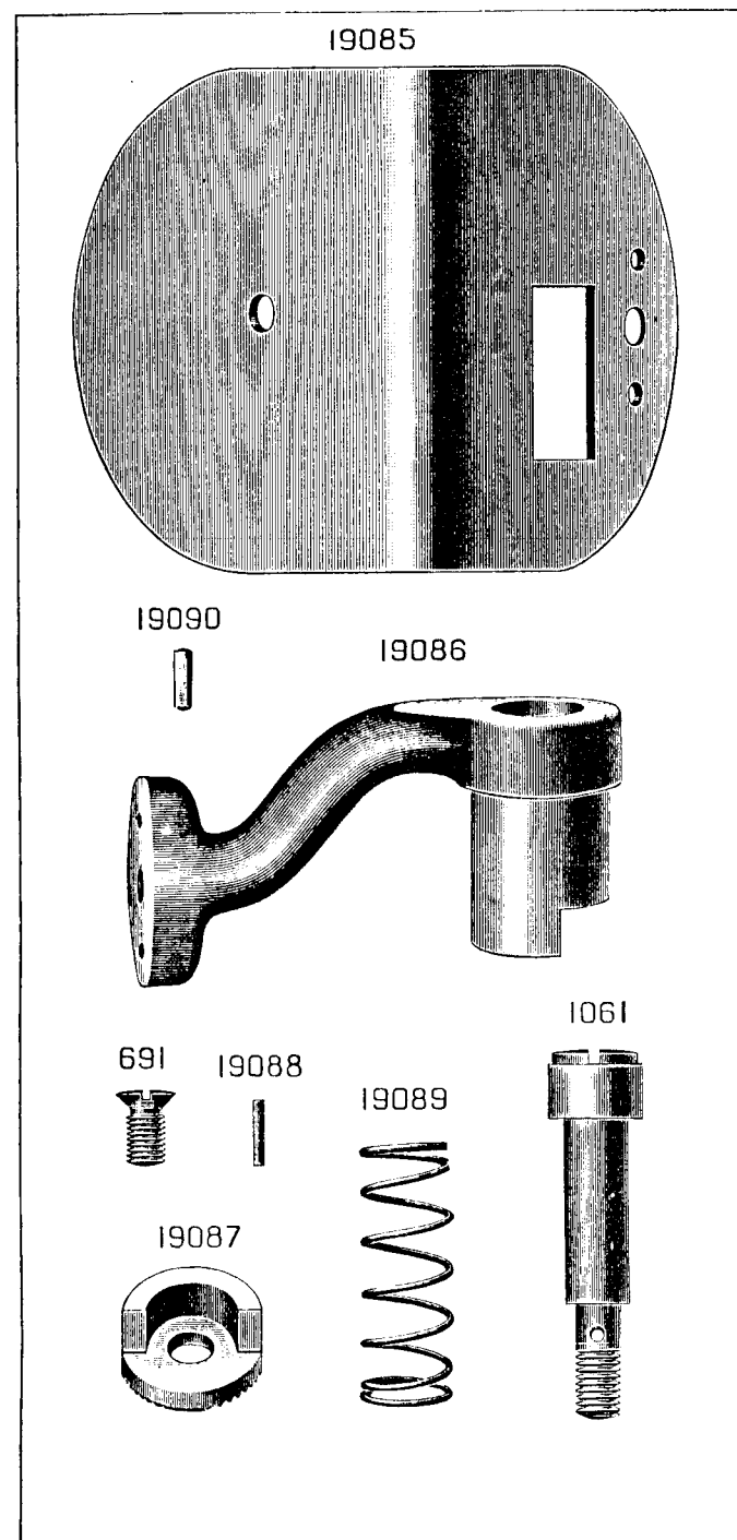
PLATE 2162—FULL SIZE
