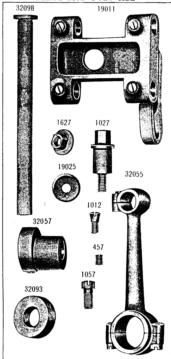
PLATE 2192—FULL SIZE
