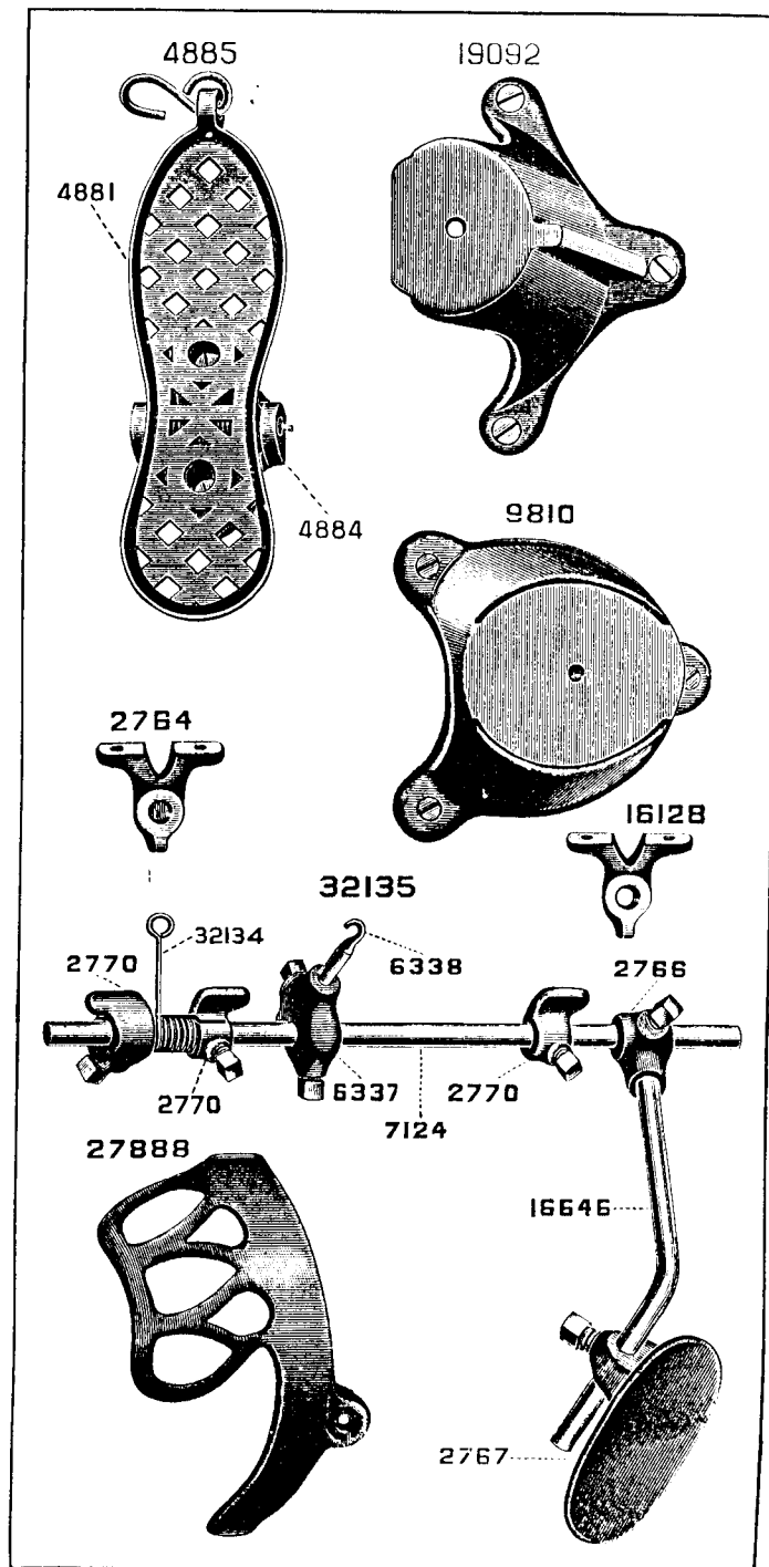
PLATE 2166—ONE-FOURTH SIZE
