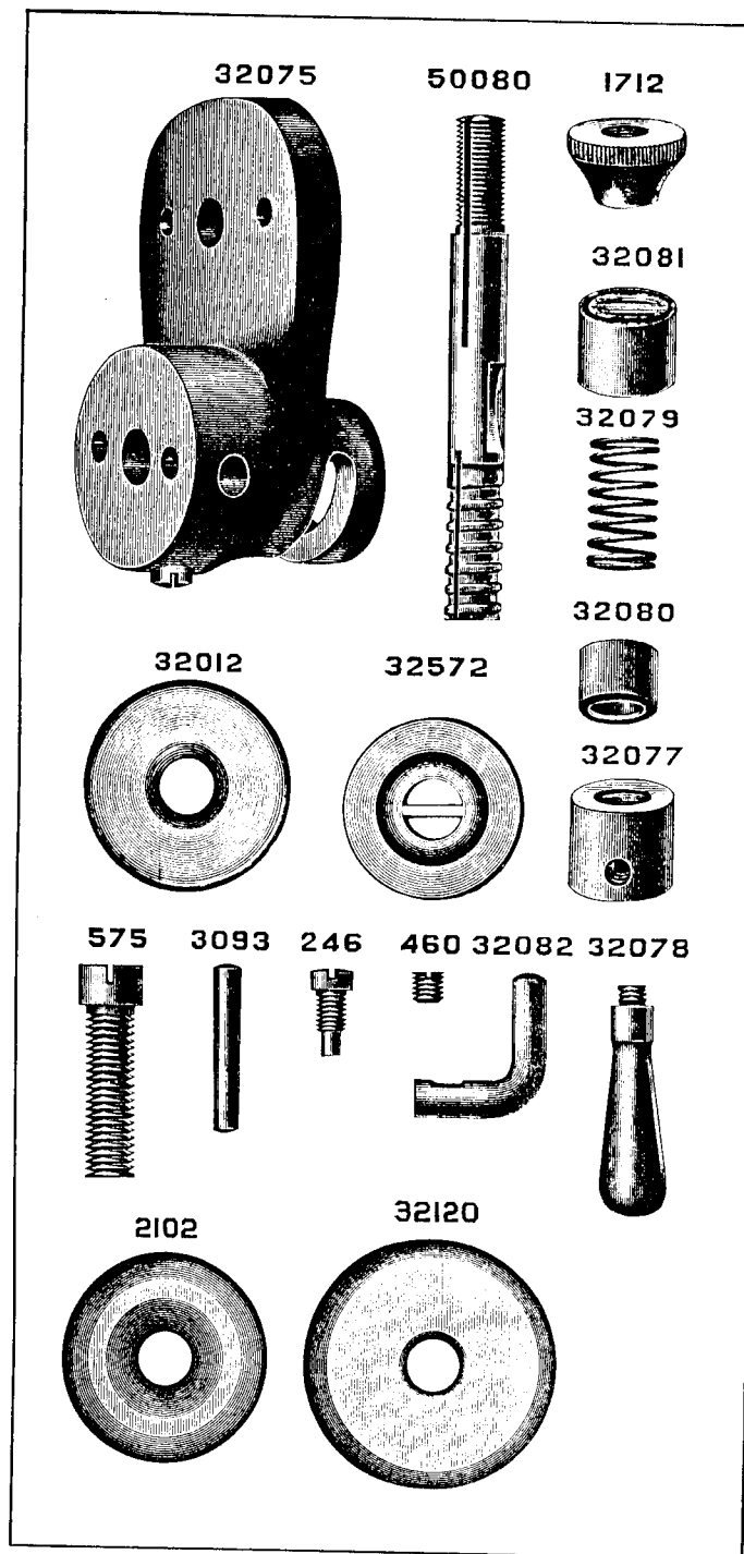
PLATE 2171—FULL SIZE
