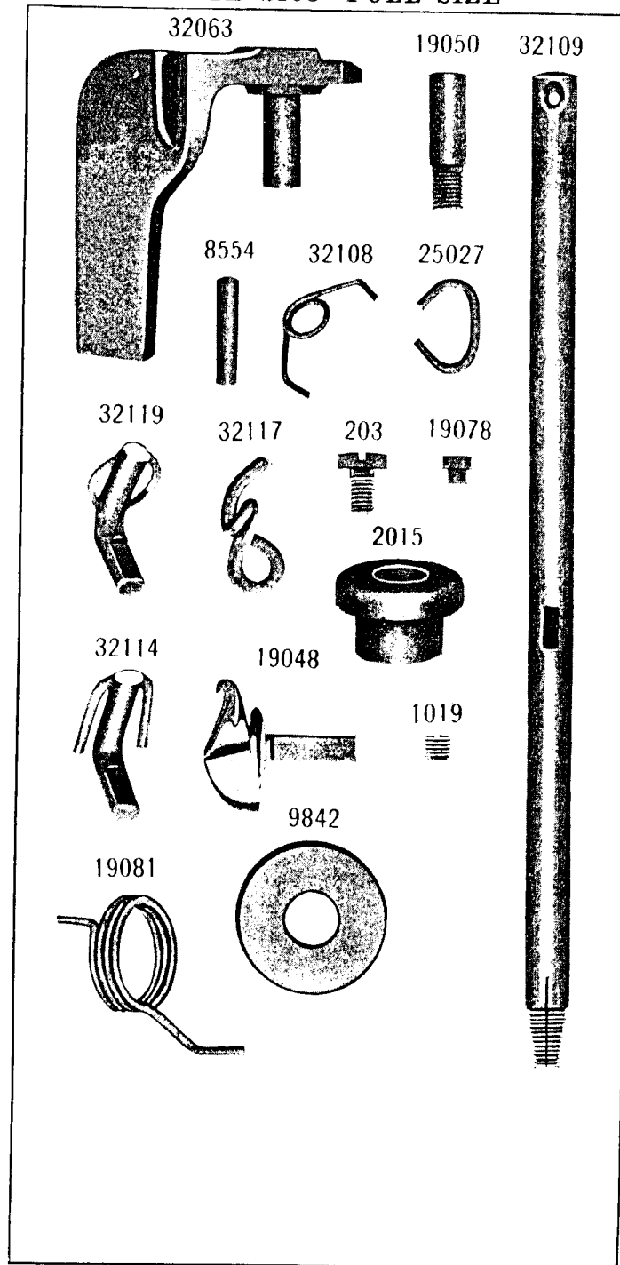
PLATE 2193—FULL SIZE
