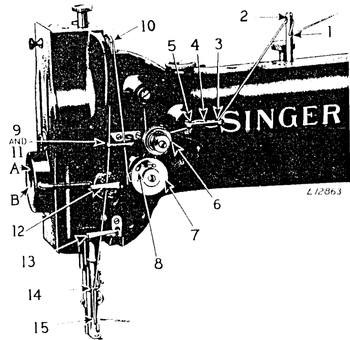
Fig. 13. Upper Threading
