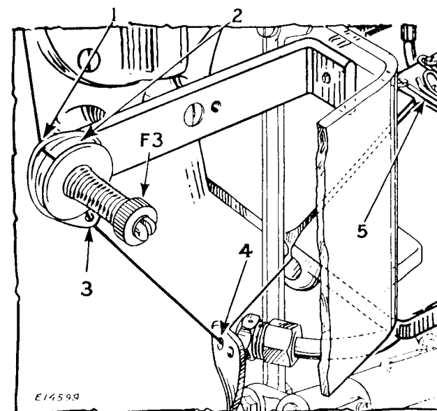
Fig. 6. Threading the Looper on Machine 147-88
