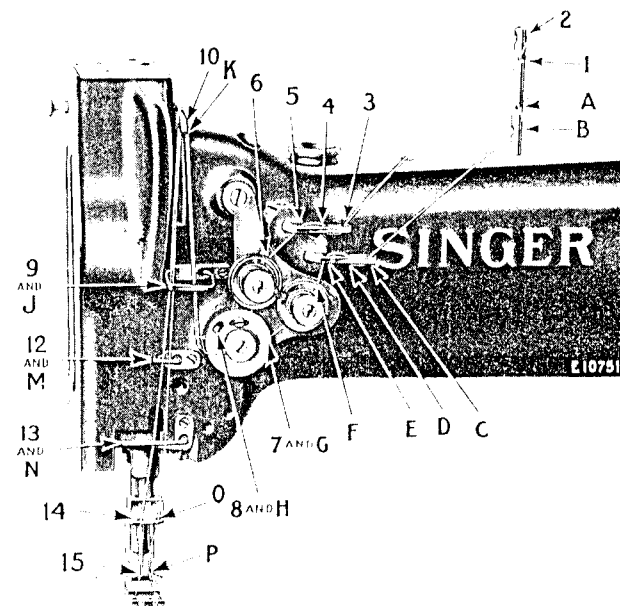
Fig. 13. Upper Threading
