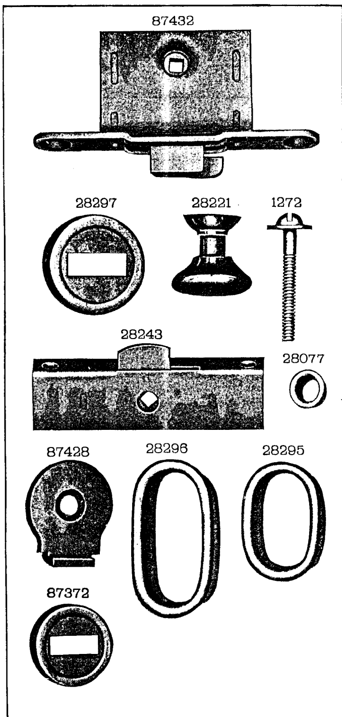
PLATE 6316 — FULL SIZE
