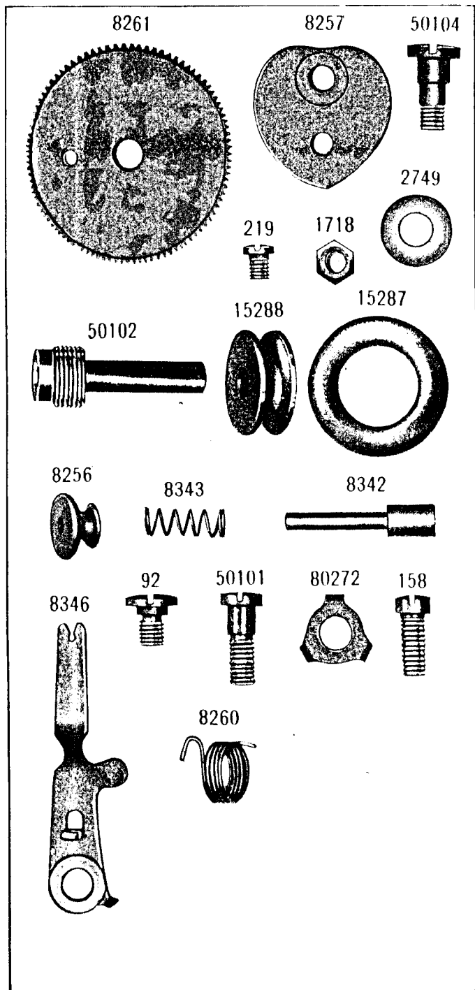
PLATE 6409—FULL SIZE
