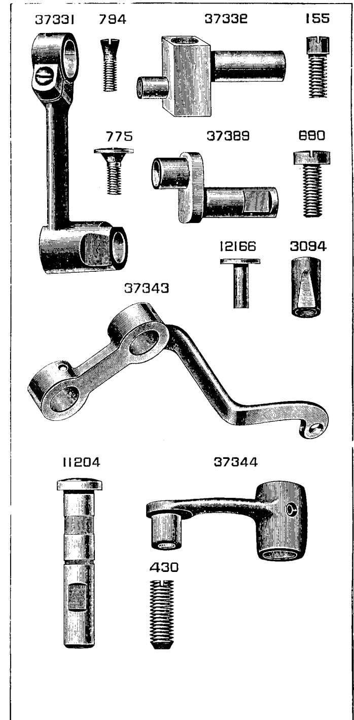
PLATE 6112—FULL SIZE
