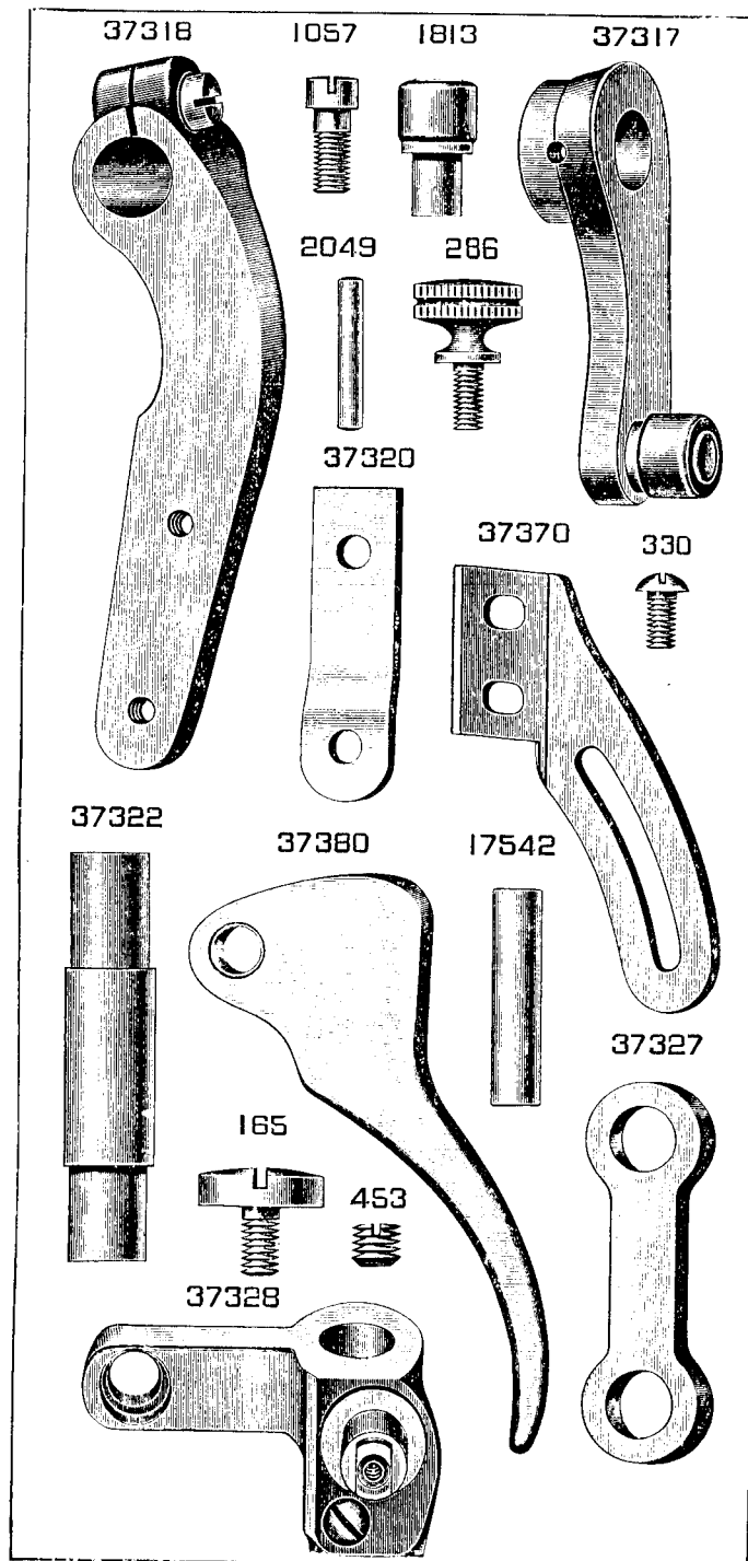
PLATE 6104—FULL SIZE
