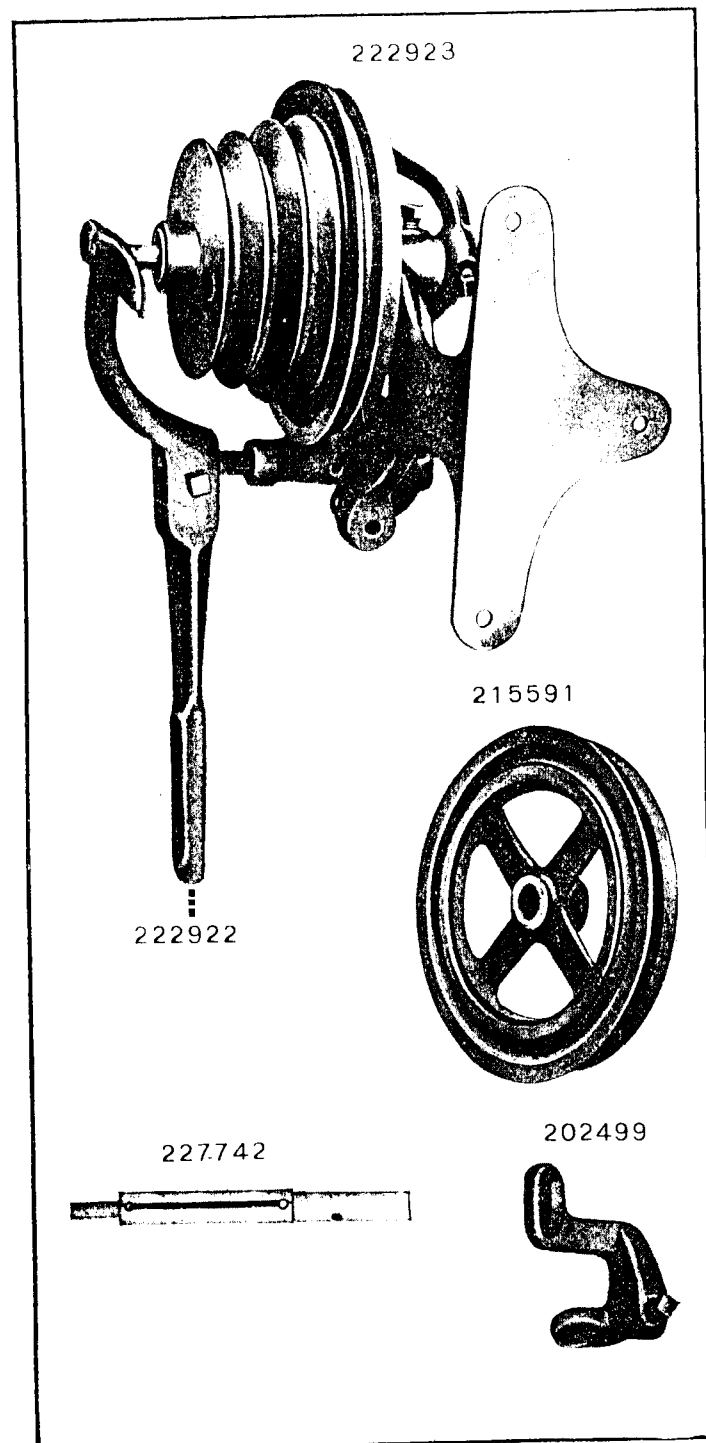
PLATE 12620-ONE-FOURTH SIZE
