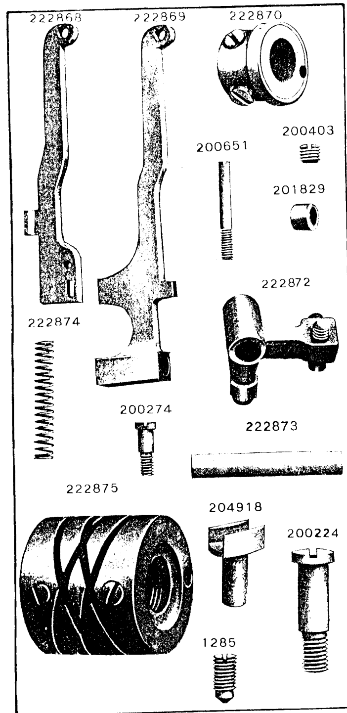
PLATE 12612 -FULL SIZE
